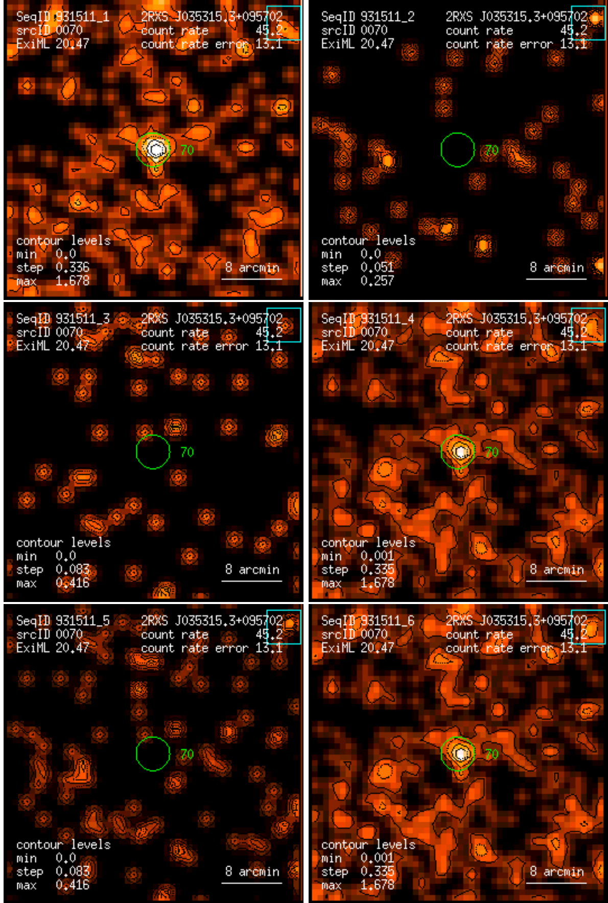
Figure 70: RASS 931511: detection 0070: band rate images, Gaussian filter: (1) PSPC channels 11 – 41, (2) 52 – 90, (3) 91 – 201, (4) 11 – 235, (5) 52 – 201, (6) 11 – 201. Broad band rates in counts/ks. Band rate contour levels in counts/ks/arcmin 2 .
