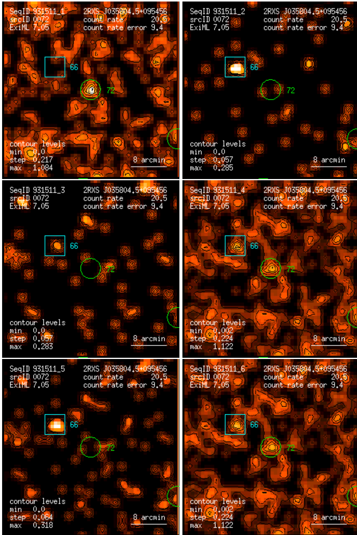
Figure 72: RASS 931511: detection 0072: band rate images, Gaussian filter: (1) PSPC channels 11 – 41, (2) 52 – 90, (3) 91 – 201, (4) 11 – 235, (5) 52 – 201, (6) 11 – 201. Broad band rates in counts/ks. Band rate contour levels in counts/ks/arcmin 2 .
