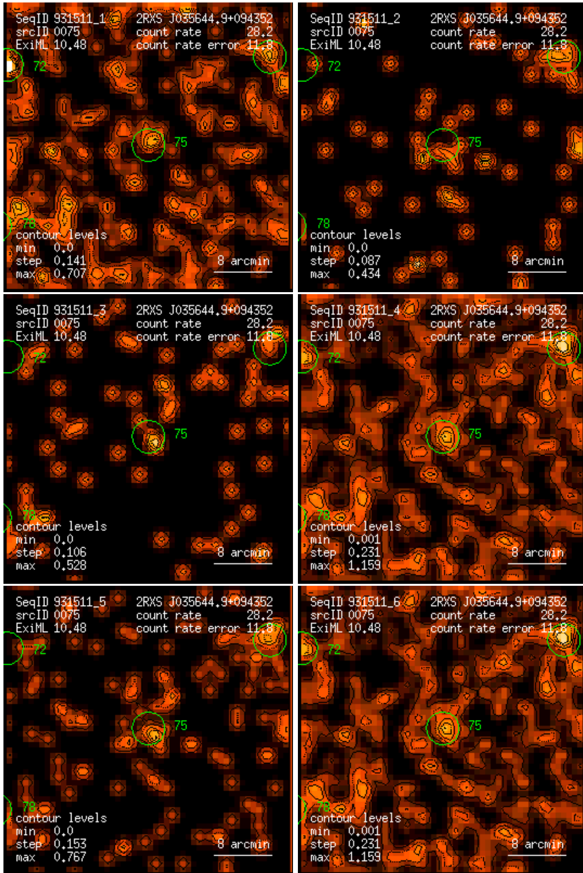
Figure 75: RASS 931511: detection 0075: band rate images, Gaussian filter: (1) PSPC channels 11 – 41, (2) 52 – 90, (3) 91 – 201, (4) 11 – 235, (5) 52 – 201, (6) 11 – 201. Broad band rates in counts/ks. Band rate contour levels in counts/ks/arcmin 2 .
