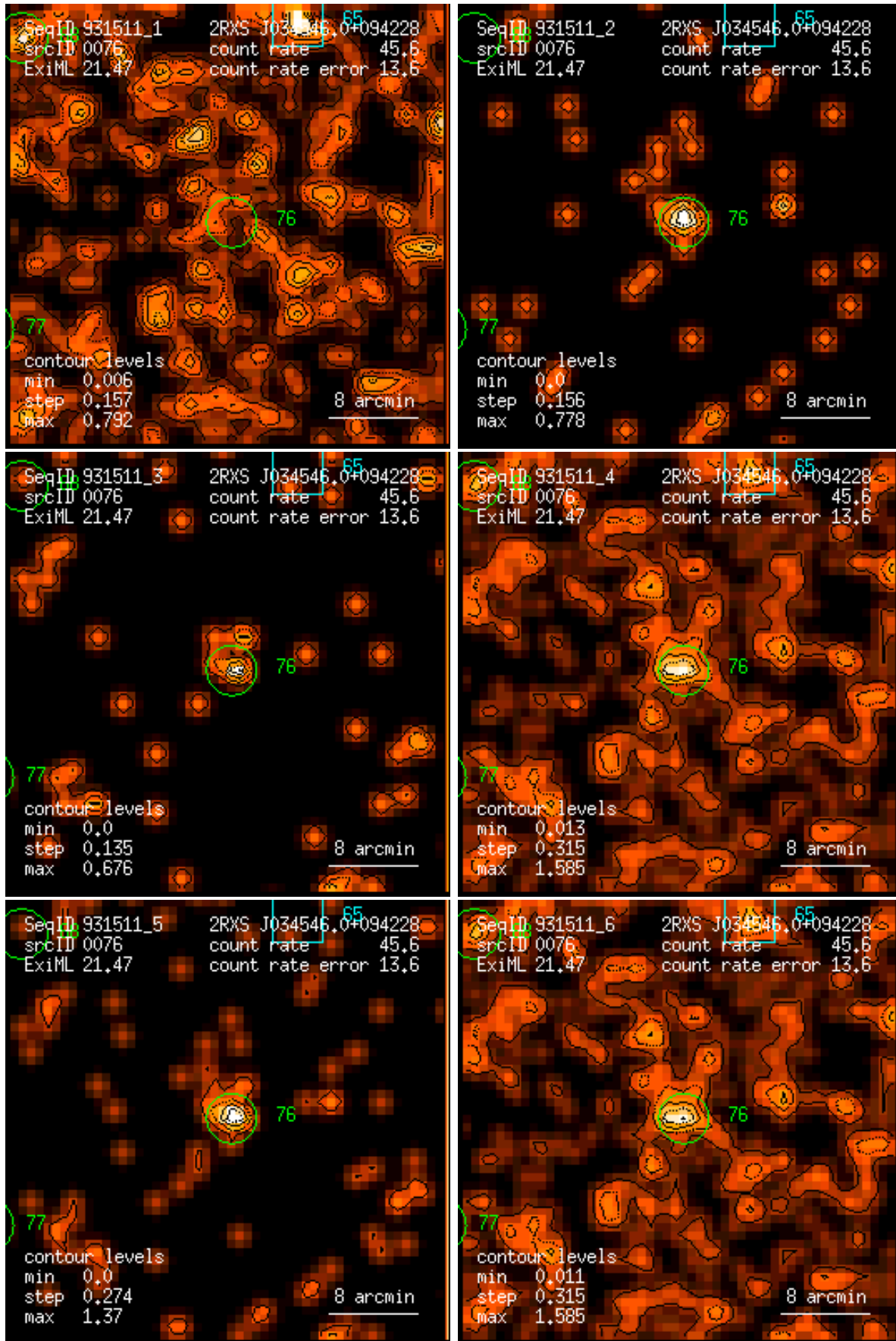
Figure 76: RASS 931511: detection 0076: band rate images, Gaussian filter: (1) PSPC channels 11 – 41, (2) 52 – 90, (3) 91 – 201, (4) 11 – 235, (5) 52 – 201, (6) 11 – 201. Broad band rates in counts/ks. Band rate contour levels in counts/ks/arcmin 2 .
