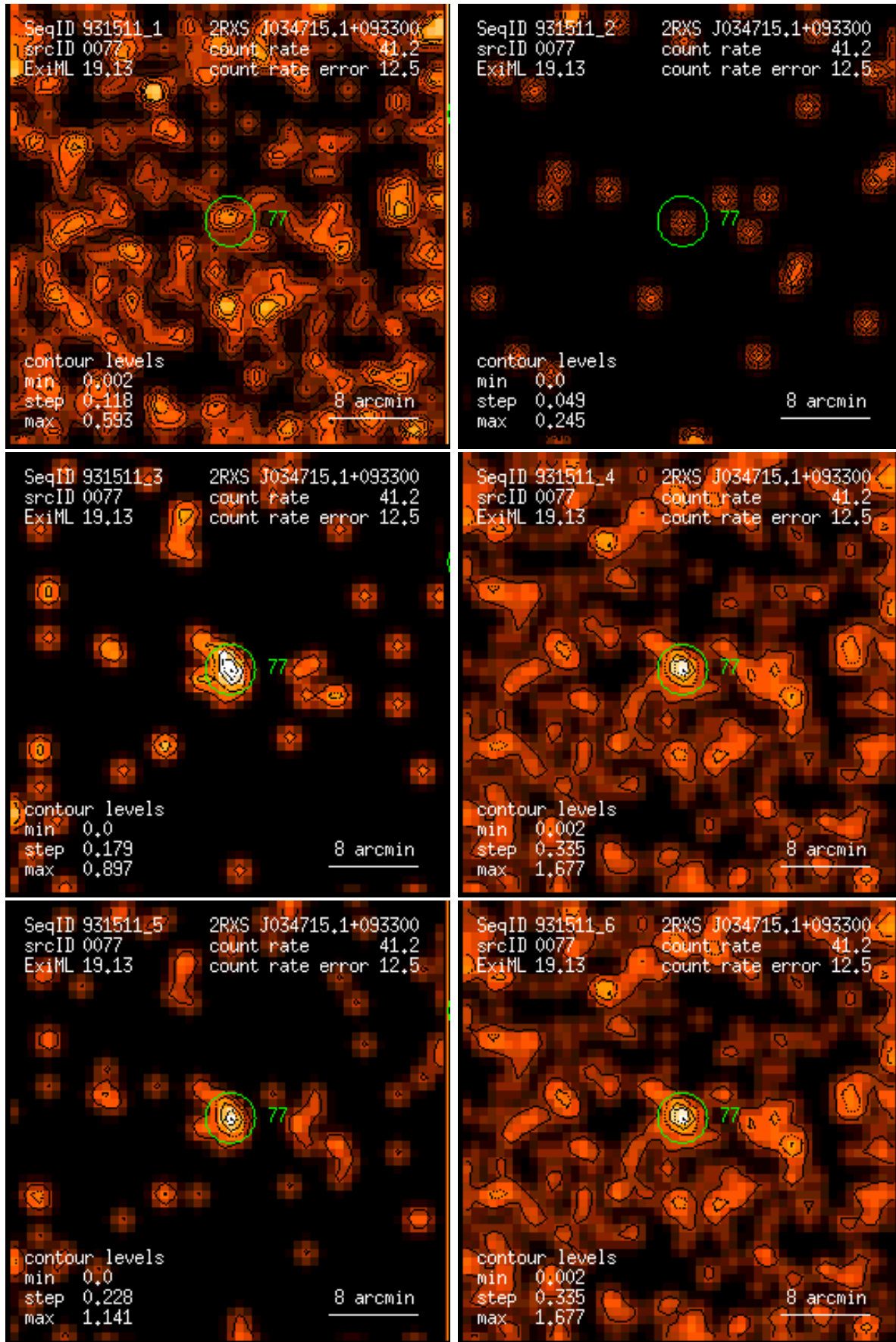
Figure 77: RASS 931511: detection 0077: band rate images, Gaussian filter: (1) PSPC channels 11 – 41, (2) 52 – 90, (3) 91 – 201, (4) 11 – 235, (5) 52 – 201, (6) 11 – 201. Broad band rates in counts/ks. Band rate contour levels in counts/ks/arcmin 2 .
