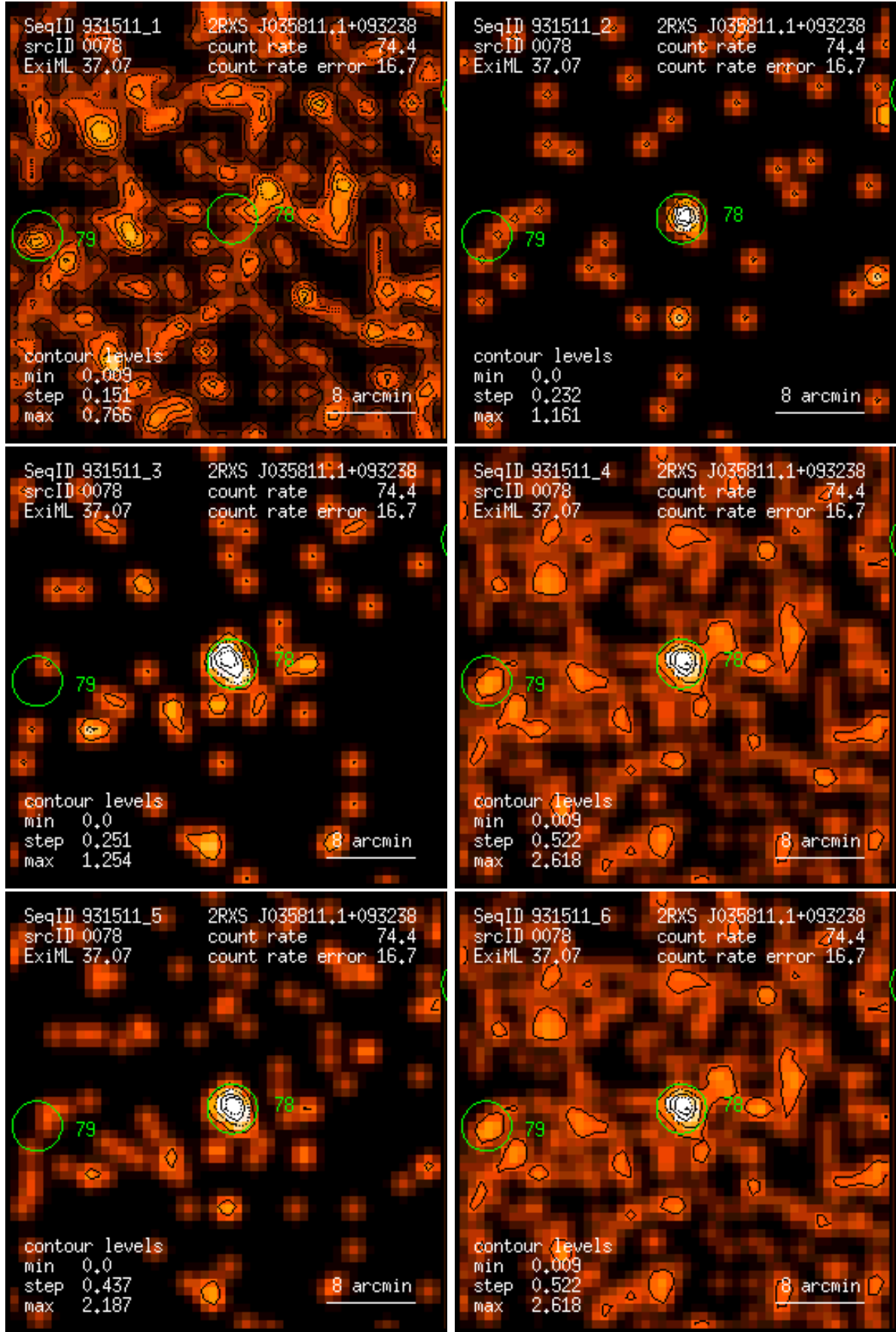
Figure 78: RASS 931511: detection 0078: band rate images, Gaussian filter: (1) PSPC channels 11 – 41, (2) 52 – 90, (3) 91 – 201, (4) 11 – 235, (5) 52 – 201, (6) 11 – 201. Broad band rates in counts/ks. Band rate contour levels in counts/ks/arcmin 2 .
