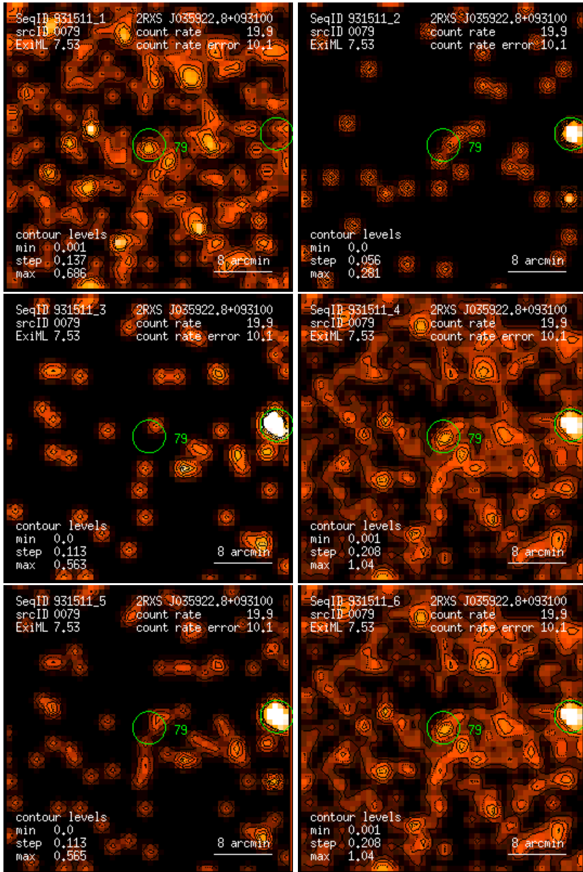
Figure 79: RASS 931511: detection 0079: band rate images, Gaussian filter: (1) PSPC channels 11 – 41, (2) 52 – 90, (3) 91 – 201, (4) 11 – 235, (5) 52 – 201, (6) 11 – 201. Broad band rates in counts/ks. Band rate contour levels in counts/ks/arcmin 2 .
