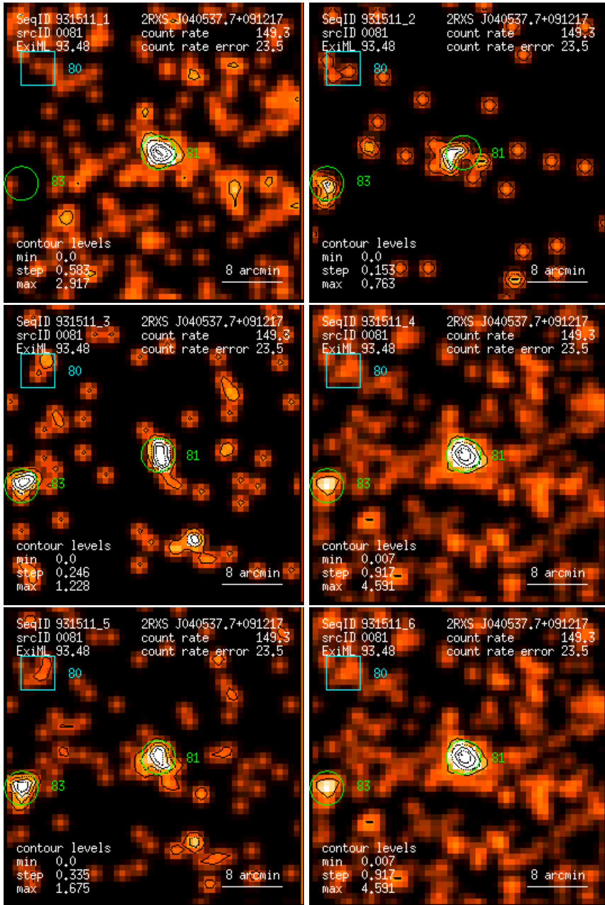
Figure 81: RASS 931511: detection 0081: band rate images, Gaussian filter: (1) PSPC channels 11 – 41, (2) 52 – 90, (3) 91 – 201, (4) 11 – 235, (5) 52 – 201, (6) 11 – 201. Broad band rates in counts/ks. Band rate contour levels in counts/ks/arcmin 2 .
