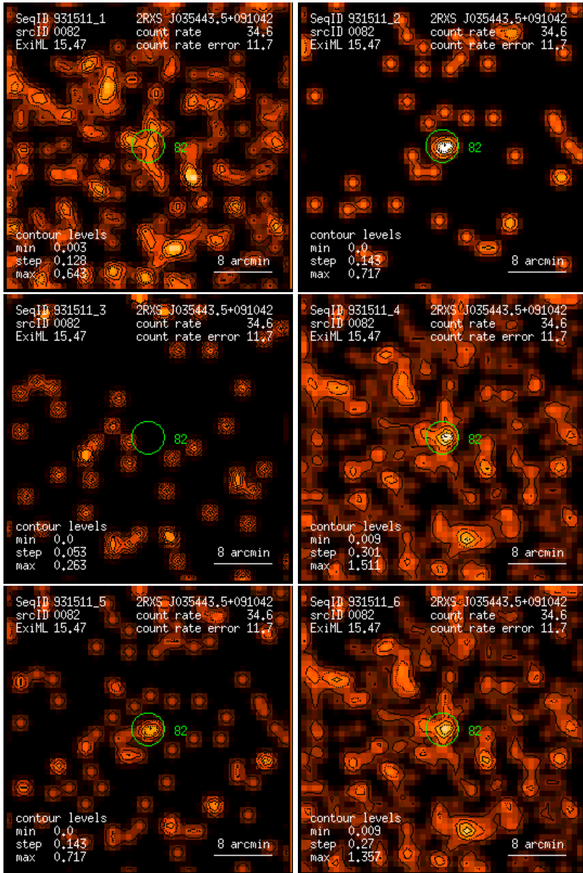
Figure 82: RASS 931511: detection 0082: band rate images, Gaussian filter: (1) PSPC channels 11 – 41, (2) 52 – 90, (3) 91 – 201, (4) 11 – 235, (5) 52 – 201, (6) 11 – 201. Broad band rates in counts/ks. Band rate contour levels in counts/ks/arcmin 2 .
