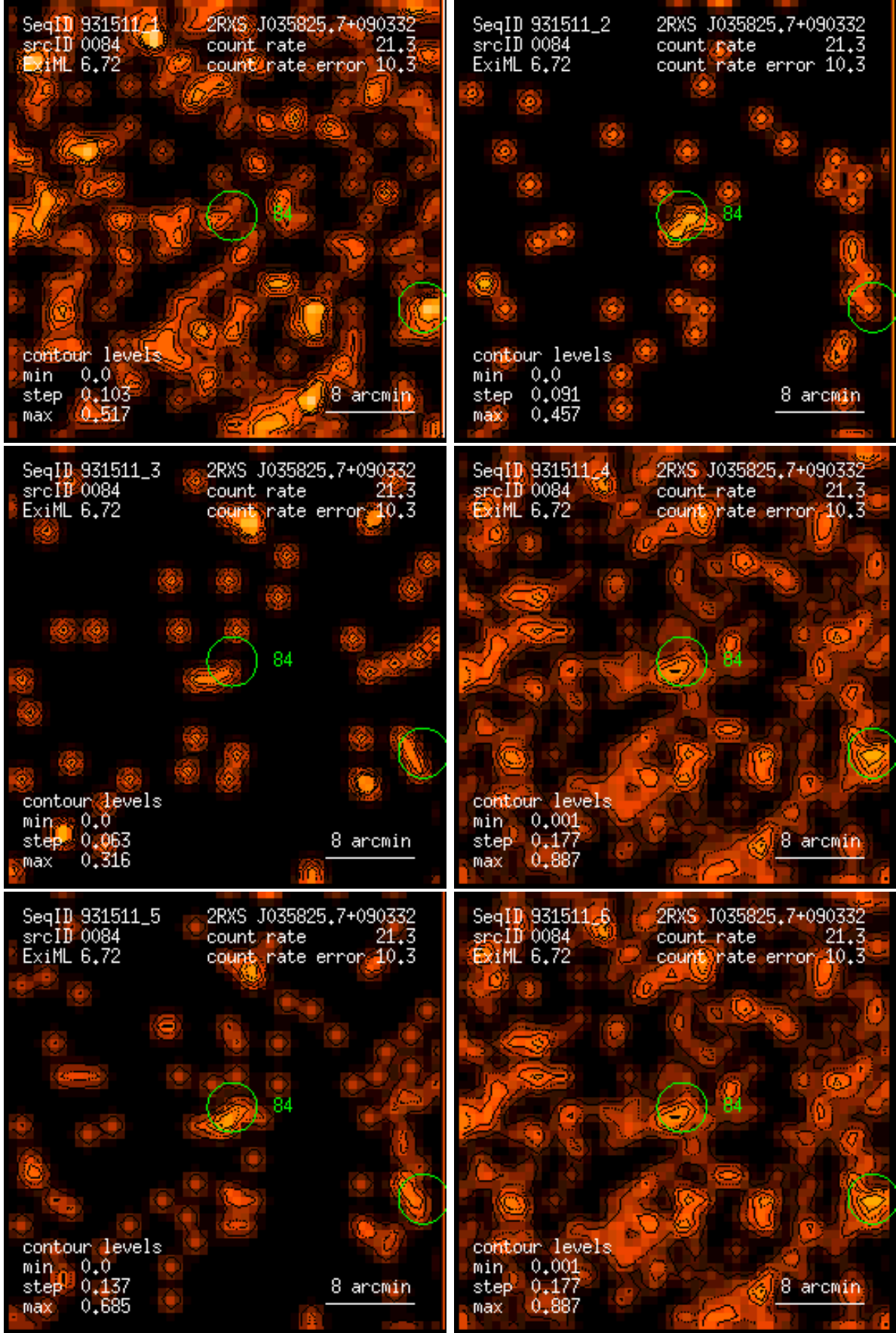
Figure 84: RASS 931511: detection 0084: band rate images, Gaussian filter: (1) PSPC channels 11 – 41, (2) 52 – 90, (3) 91 – 201, (4) 11 – 235, (5) 52 – 201, (6) 11 – 201. Broad band rates in counts/ks. Band rate contour levels in counts/ks/arcmin 2 .
