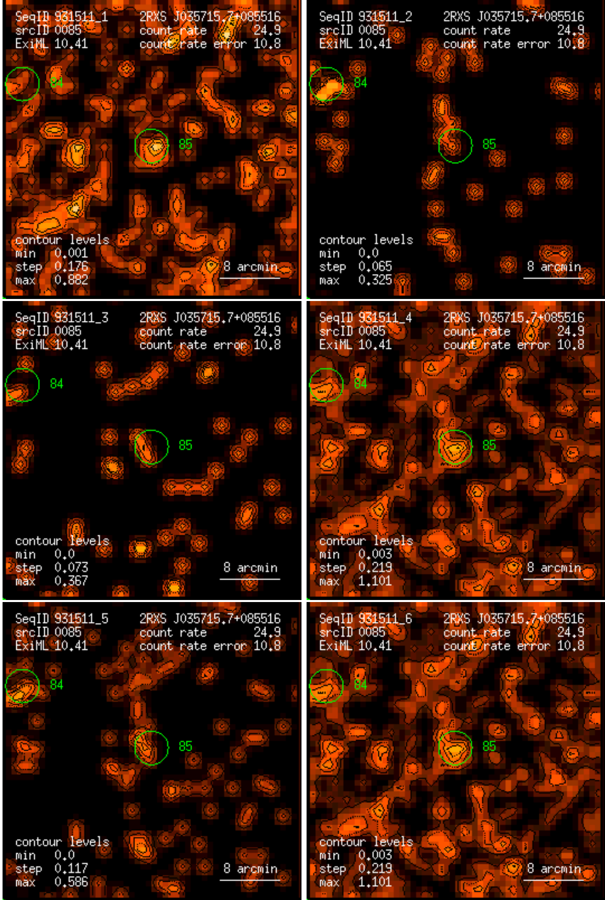
Figure 85: RASS 931511: detection 0085: band rate images, Gaussian filter: (1) PSPC channels 11 – 41, (2) 52 – 90, (3) 91 – 201, (4) 11 – 235, (5) 52 – 201, (6) 11 – 201. Broad band rates in counts/ks. Band rate contour levels in counts/ks/arcmin 2 .
