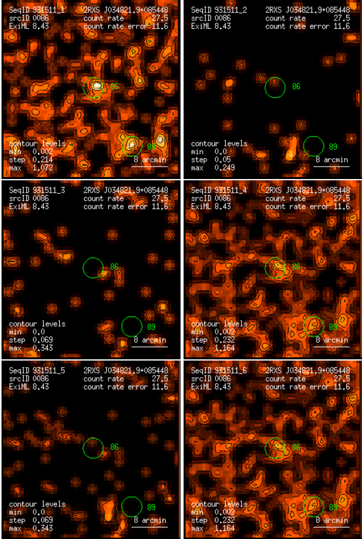
Figure 86: RASS 931511: detection 0086: band rate images, Gaussian filter: (1) PSPC channels 11 – 41, (2) 52 – 90, (3) 91 – 201, (4) 11 – 235, (5) 52 – 201, (6) 11 – 201. Broad band rates in counts/ks. Band rate contour levels in counts/ks/arcmin 2 .
