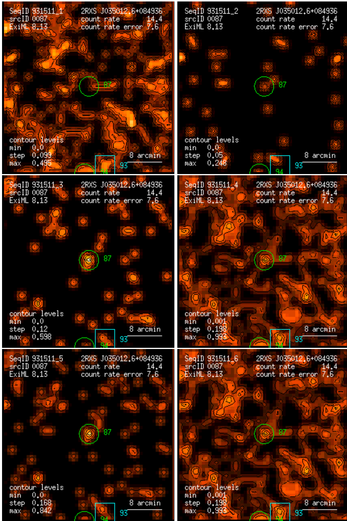
Figure 87: RASS 931511: detection 0087: band rate images, Gaussian filter: (1) PSPC channels 11 – 41, (2) 52 – 90, (3) 91 – 201, (4) 11 – 235, (5) 52 – 201, (6) 11 – 201. Broad band rates in counts/ks. Band rate contour levels in counts/ks/arcmin 2 .
