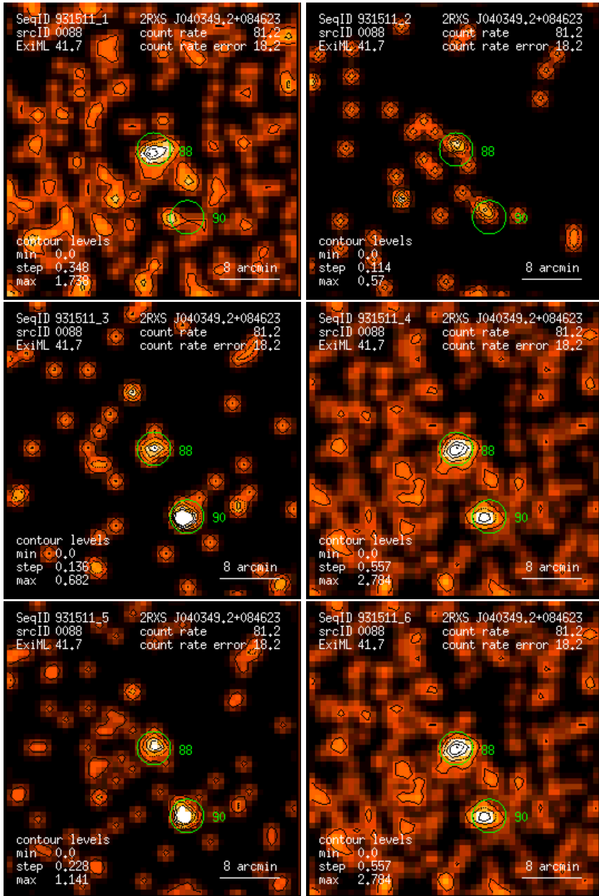
Figure 88: RASS 931511: detection 0088: band rate images, Gaussian filter: (1) PSPC channels 11 – 41, (2) 52 – 90, (3) 91 – 201, (4) 11 – 235, (5) 52 – 201, (6) 11 – 201. Broad band rates in counts/ks. Band rate contour levels in counts/ks/arcmin 2 .
