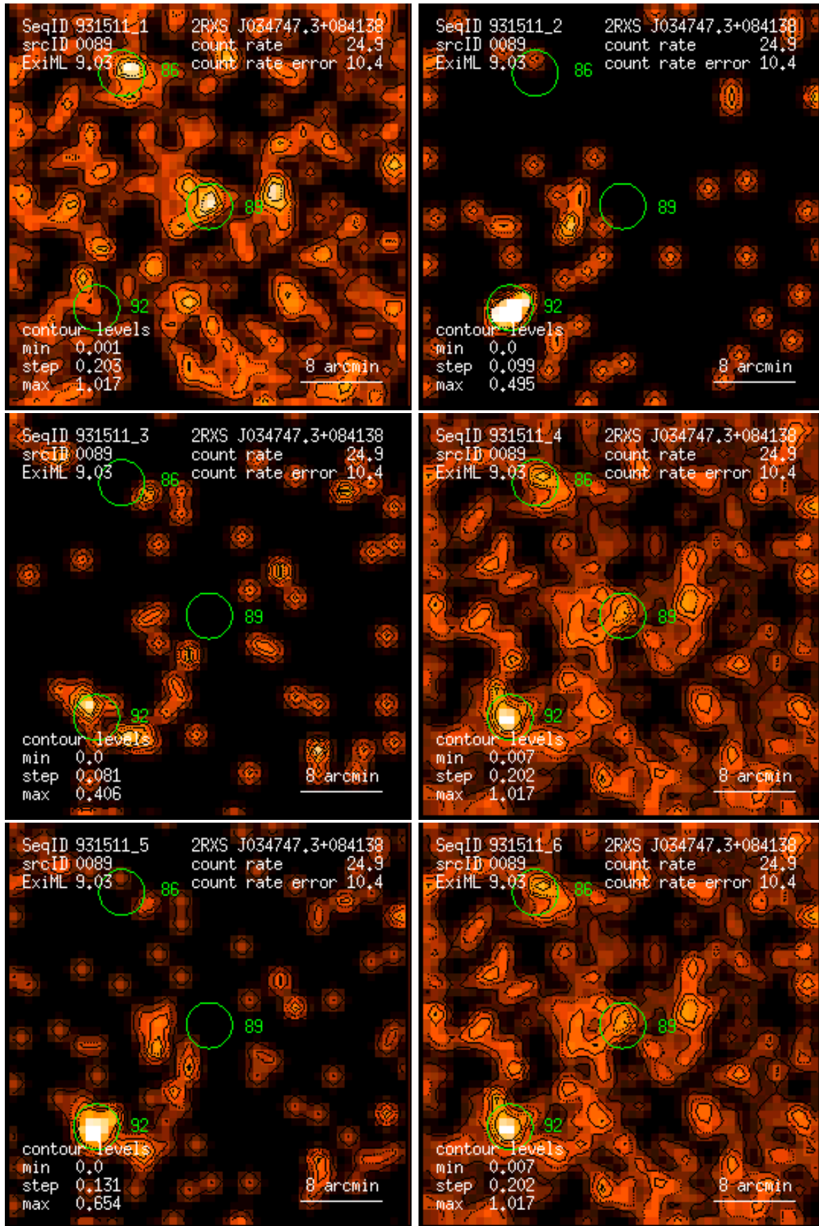
Figure 89: RASS 931511: detection 0089: band rate images, Gaussian filter: (1) PSPC channels 11 – 41, (2) 52 – 90, (3) 91 – 201, (4) 11 – 235, (5) 52 – 201, (6) 11 – 201. Broad band rates in counts/ks. Band rate contour levels in counts/ks/arcmin 2 .
