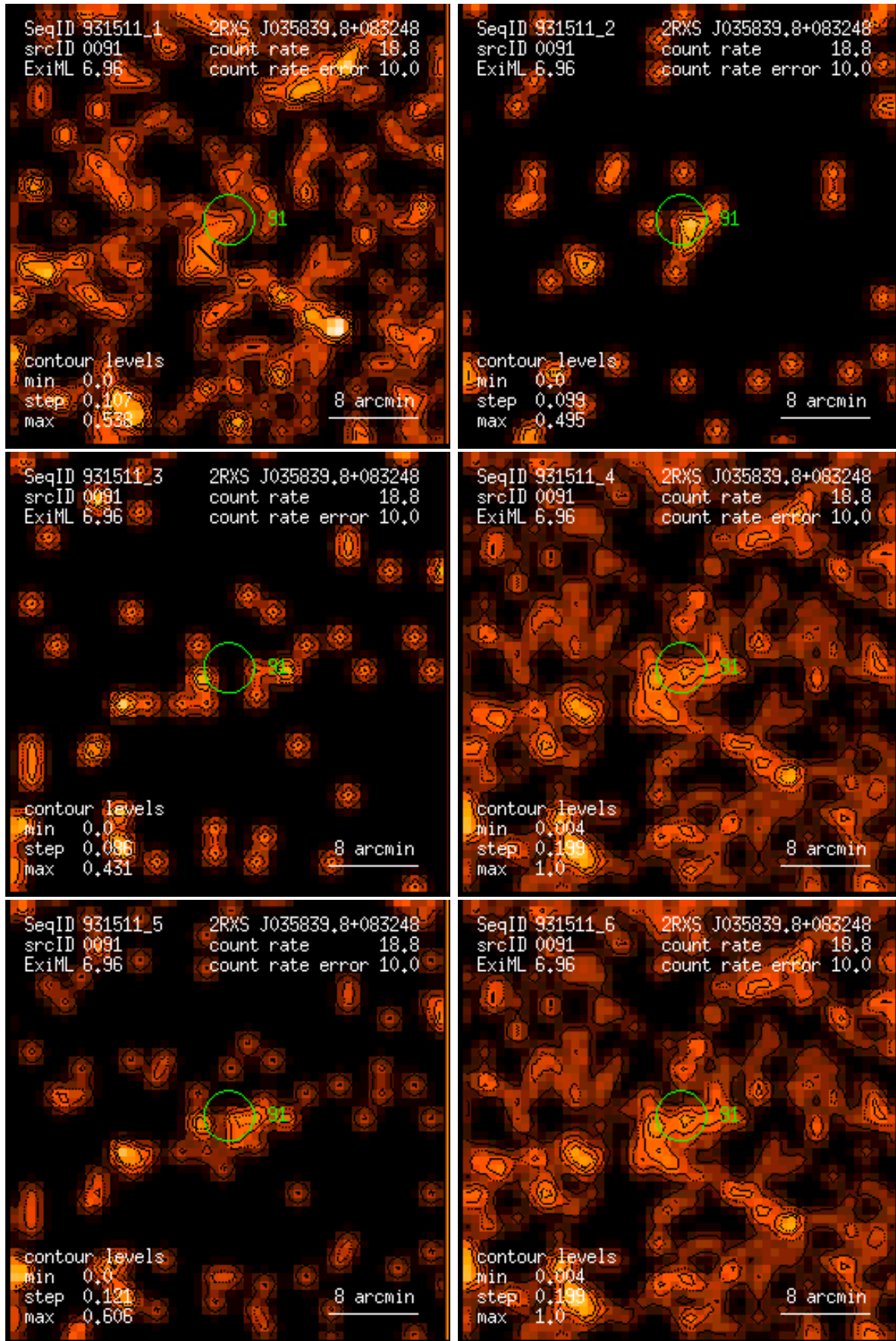
Figure 91: RASS 931511: detection 0091: band rate images, Gaussian filter: (1) PSPC channels 11 – 41, (2) 52 – 90, (3) 91 – 201, (4) 11 – 235, (5) 52 – 201, (6) 11 – 201. Broad band rates in counts/ks. Band rate contour levels in counts/ks/arcmin 2 .
