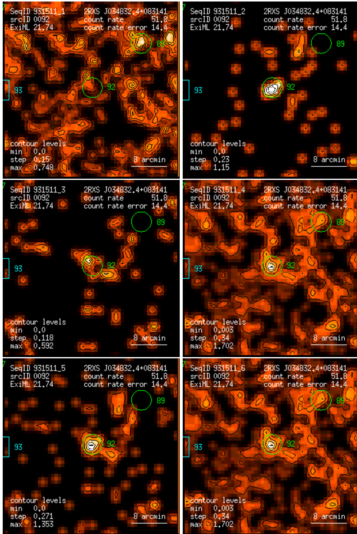
Figure 92: RASS 931511: detection 0092: band rate images, Gaussian filter: (1) PSPC channels 11 – 41, (2) 52 – 90, (3) 91 – 201, (4) 11 – 235, (5) 52 – 201, (6) 11 – 201. Broad band rates in counts/ks. Band rate contour levels in counts/ks/arcmin 2 .
