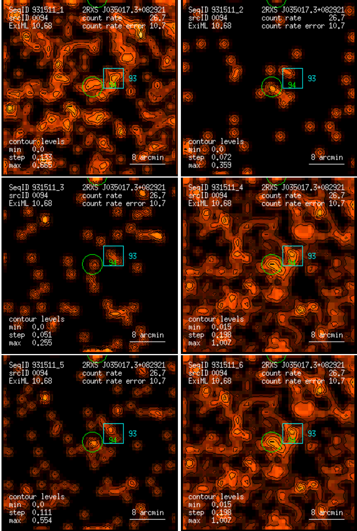
Figure 94: RASS 931511: detection 0094: band rate images, Gaussian filter: (1) PSPC channels 11 – 41, (2) 52 – 90, (3) 91 – 201, (4) 11 – 235, (5) 52 – 201, (6) 11 – 201. Broad band rates in counts/ks. Band rate contour levels in counts/ks/arcmin 2 .
