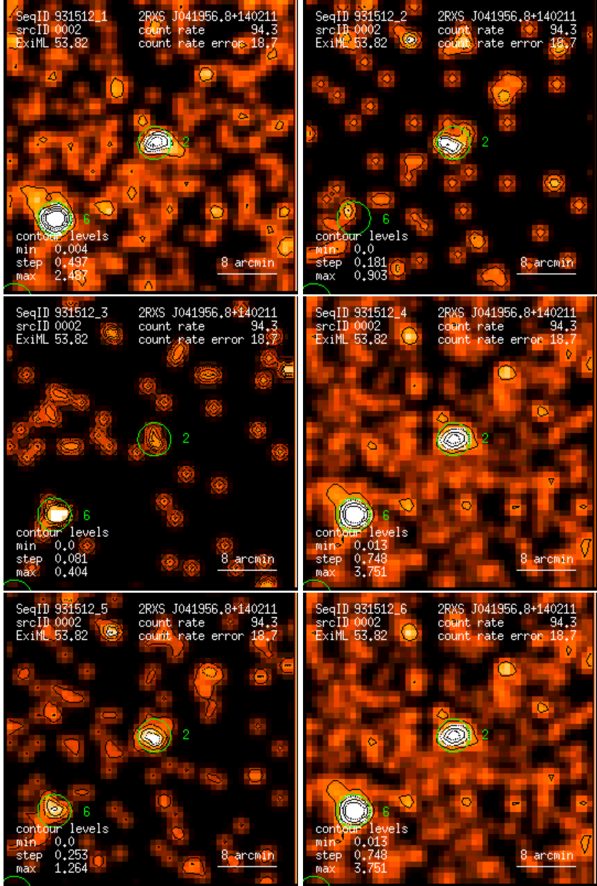
Figure 2: RASS 931512: detection 0002: band rate images, Gaussian filter: (1) PSPC channels 11 – 41, (2) 52 – 90, (3) 91 – 201, (4) 11 – 235, (5) 52 – 201, (6) 11 – 201. Broad band rates in counts/ks. Band rate contour levels in counts/ks/arcmin 2 .
