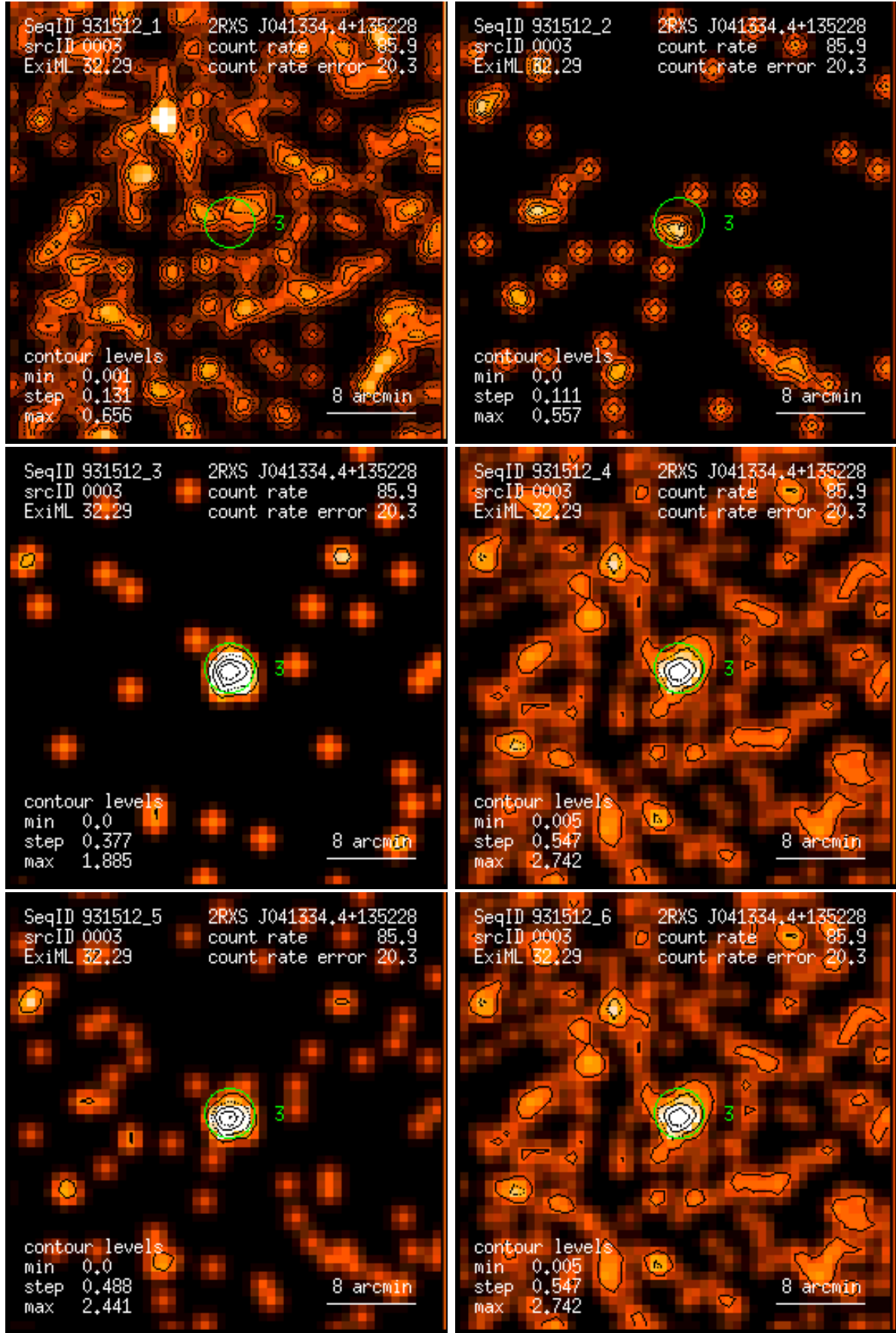
Figure 3: RASS 931512: detection 0003: band rate images, Gaussian filter: (1) PSPC channels 11 – 41, (2) 52 – 90, (3) 91 – 201, (4) 11 – 235, (5) 52 – 201, (6) 11 – 201. Broad band rates in counts/ks. Band rate contour levels in counts/ks/arcmin 2 .
