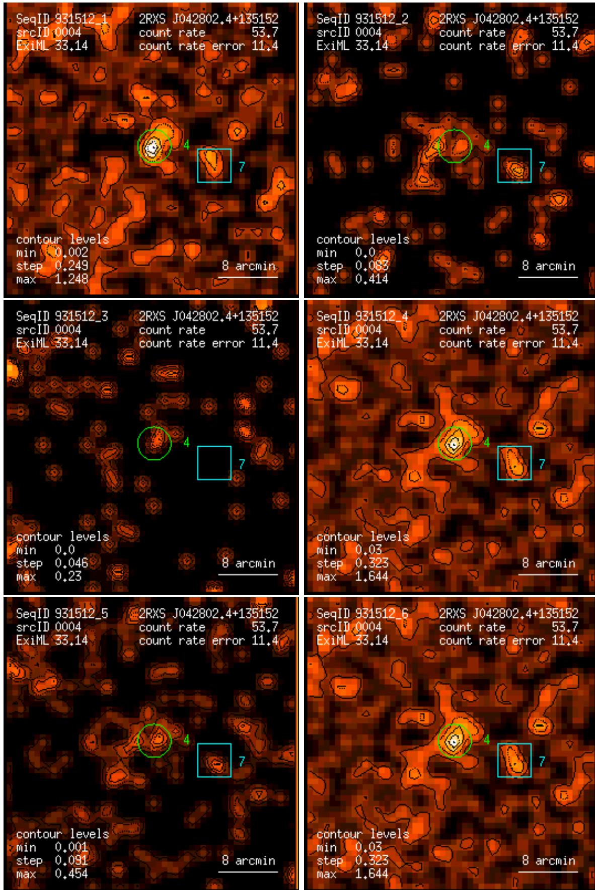
Figure 4: RASS 931512: detection 0004: band rate images, Gaussian filter: (1) PSPC channels 11 – 41, (2) 52 – 90, (3) 91 – 201, (4) 11 – 235, (5) 52 – 201, (6) 11 – 201. Broad band rates in counts/ks. Band rate contour levels in counts/ks/arcmin 2 .
