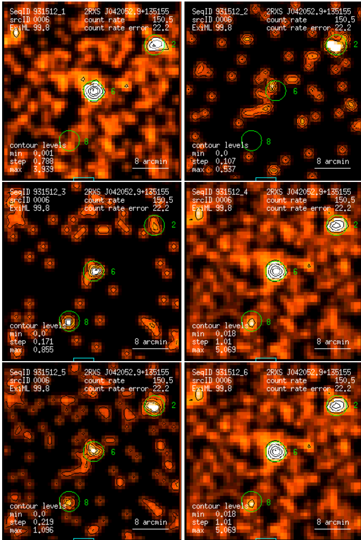
Figure 6: RASS 931512: detection 0006: band rate images, Gaussian filter: (1) PSPC channels 11 – 41, (2) 52 – 90, (3) 91 – 201, (4) 11 – 235, (5) 52 – 201, (6) 11 – 201. Broad band rates in counts/ks. Band rate contour levels in counts/ks/arcmin 2 .
