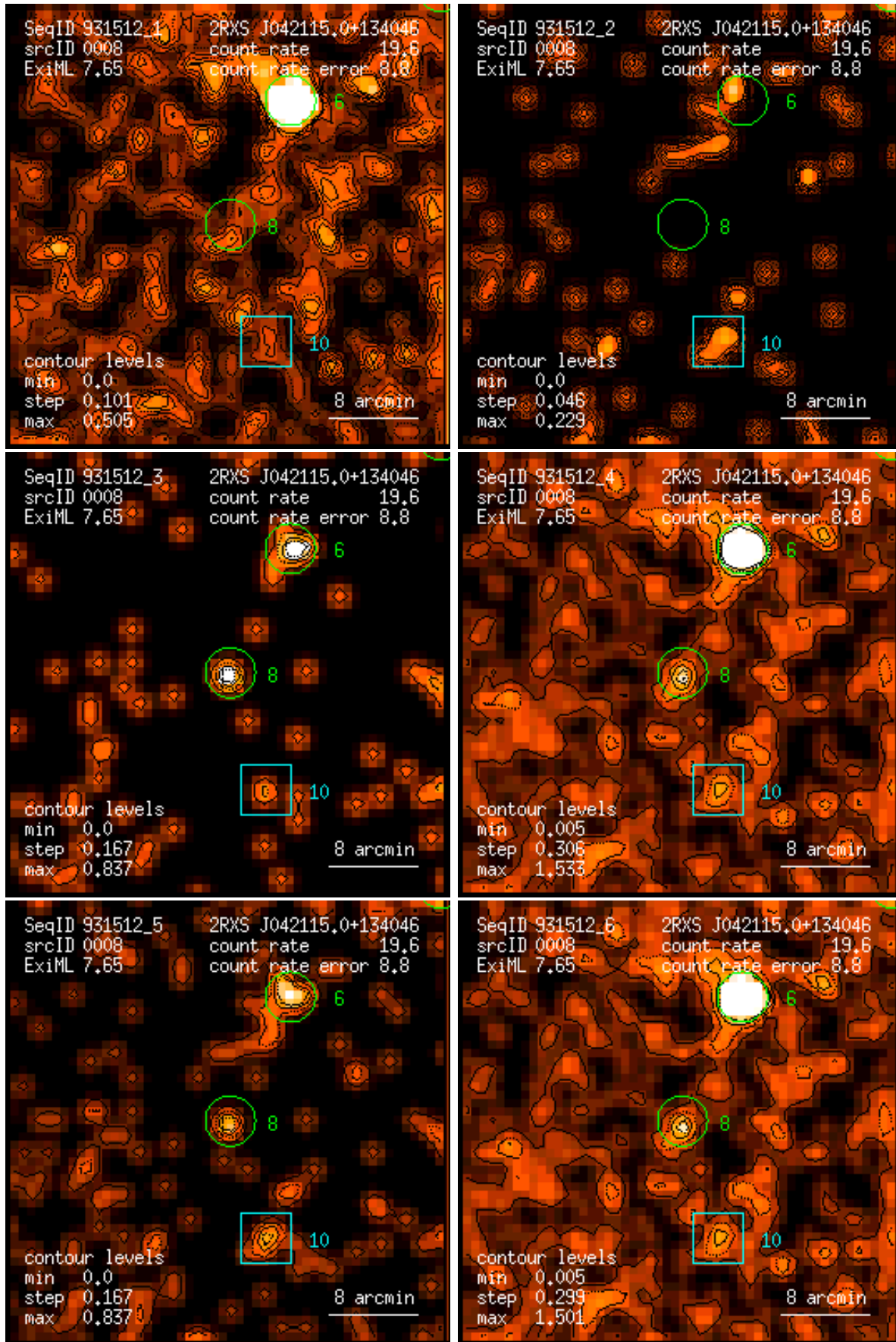
Figure 8: RASS 931512: detection 0008: band rate images, Gaussian filter: (1) PSPC channels 11 – 41, (2) 52 – 90, (3) 91 – 201, (4) 11 – 235, (5) 52 – 201, (6) 11 – 201. Broad band rates in counts/ks. Band rate contour levels in counts/ks/arcmin 2 .
