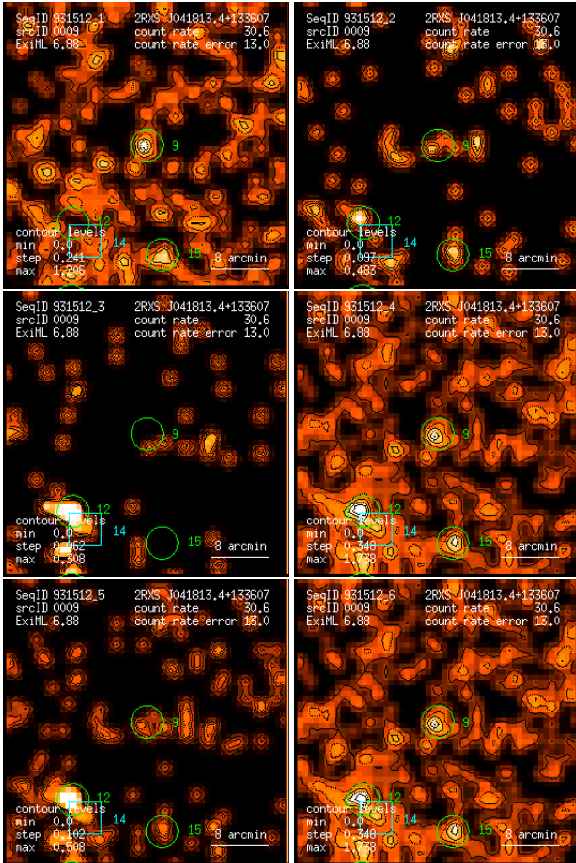
Figure 9: RASS 931512: detection 0009: band rate images, Gaussian filter: (1) PSPC channels 11 – 41, (2) 52 – 90, (3) 91 – 201, (4) 11 – 235, (5) 52 – 201, (6) 11 – 201. Broad band rates in counts/ks. Band rate contour levels in counts/ks/arcmin 2 .
