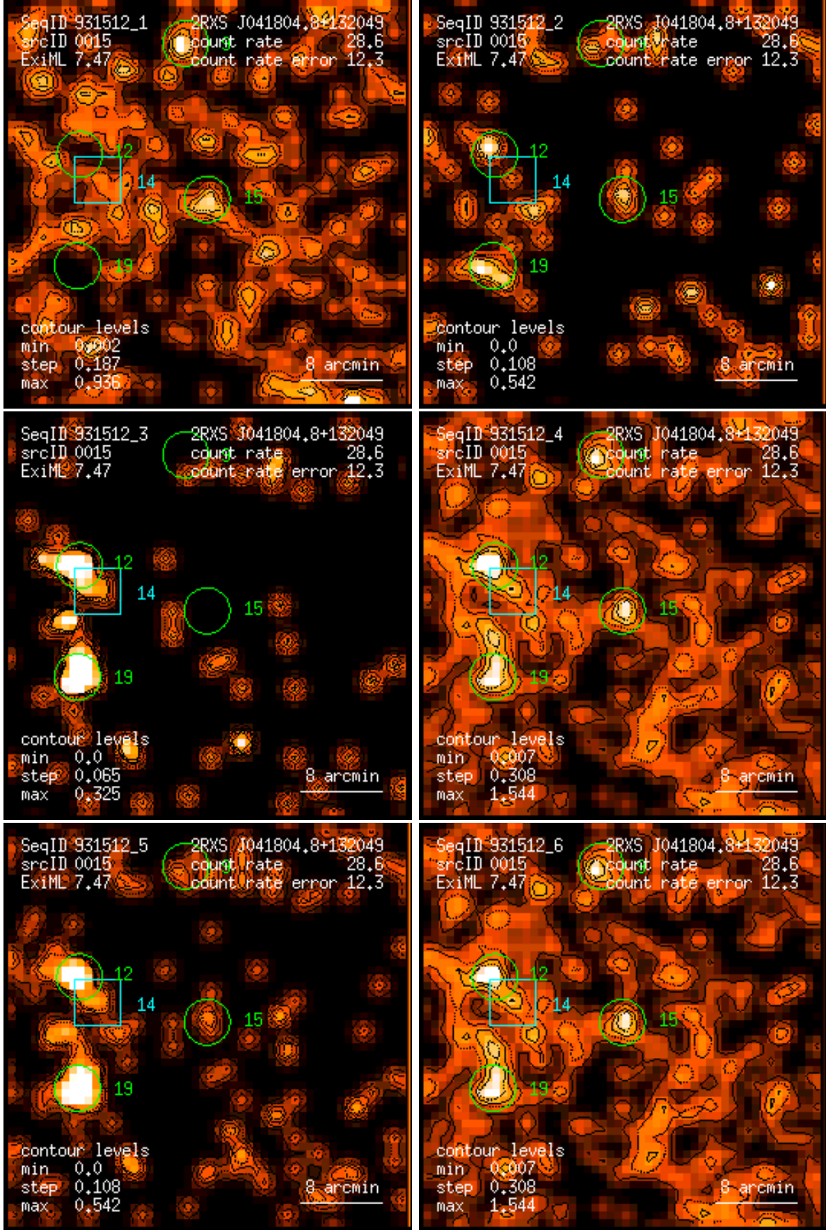
Figure 15: RASS 931512: detection 0015: band rate images, Gaussian filter: (1) PSPC channels 11 – 41, (2) 52 – 90, (3) 91 – 201, (4) 11 – 235, (5) 52 – 201, (6) 11 – 201. Broad band rates in counts/ks. Band rate contour levels in counts/ks/arcmin 2 .
