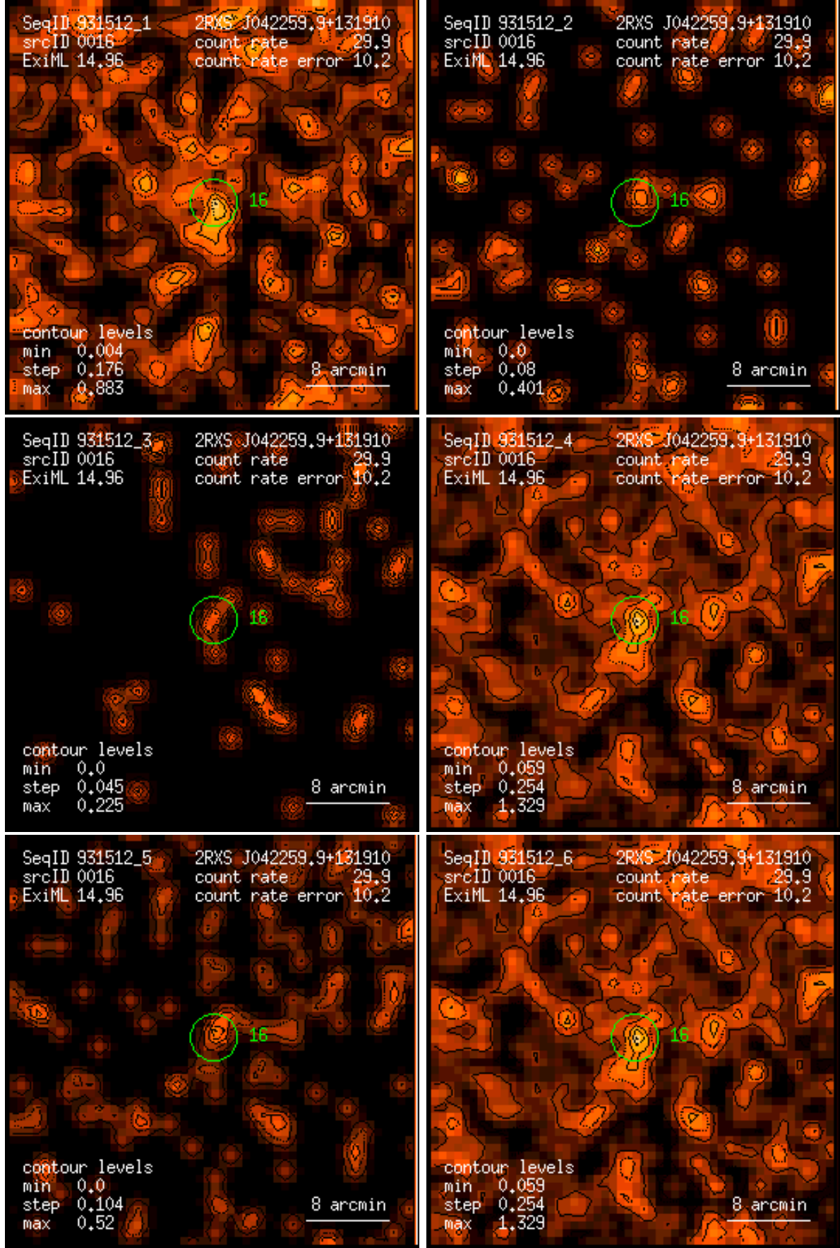
Figure 16: RASS 931512: detection 0016: band rate images, Gaussian filter: (1) PSPC channels 11 – 41, (2) 52 – 90, (3) 91 – 201, (4) 11 – 235, (5) 52 – 201, (6) 11 – 201. Broad band rates in counts/ks. Band rate contour levels in counts/ks/arcmin 2 .
