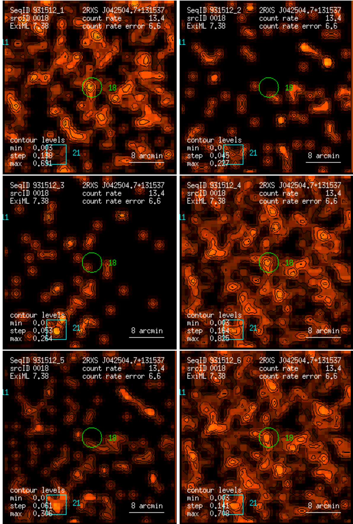
Figure 18: RASS 931512: detection 0018: band rate images, Gaussian filter: (1) PSPC channels 11 – 41, (2) 52 – 90, (3) 91 – 201, (4) 11 – 235, (5) 52 – 201, (6) 11 – 201. Broad band rates in counts/ks. Band rate contour levels in counts/ks/arcmin 2 .
