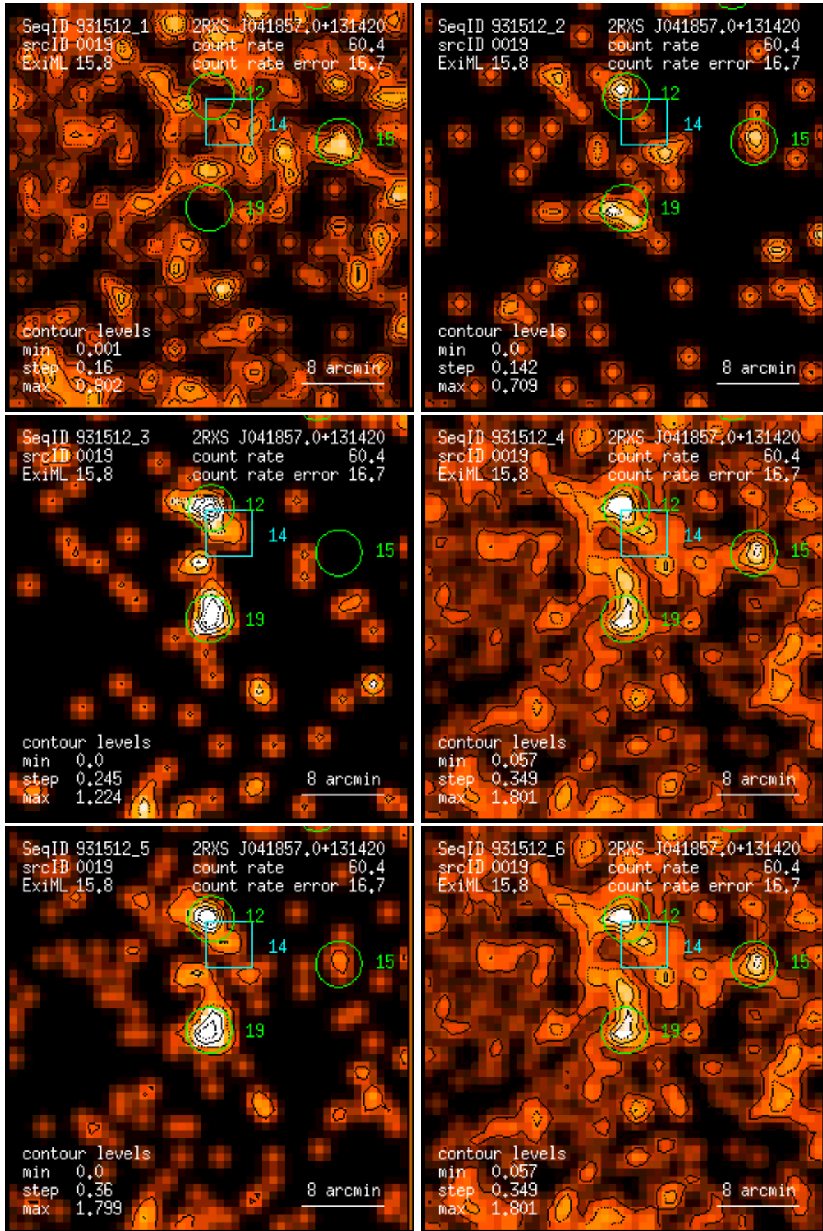
Figure 19: RASS 931512: detection 0019: band rate images, Gaussian filter: (1) PSPC channels 11 – 41, (2) 52 – 90, (3) 91 – 201, (4) 11 – 235, (5) 52 – 201, (6) 11 – 201. Broad band rates in counts/ks. Band rate contour levels in counts/ks/arcmin 2 .
