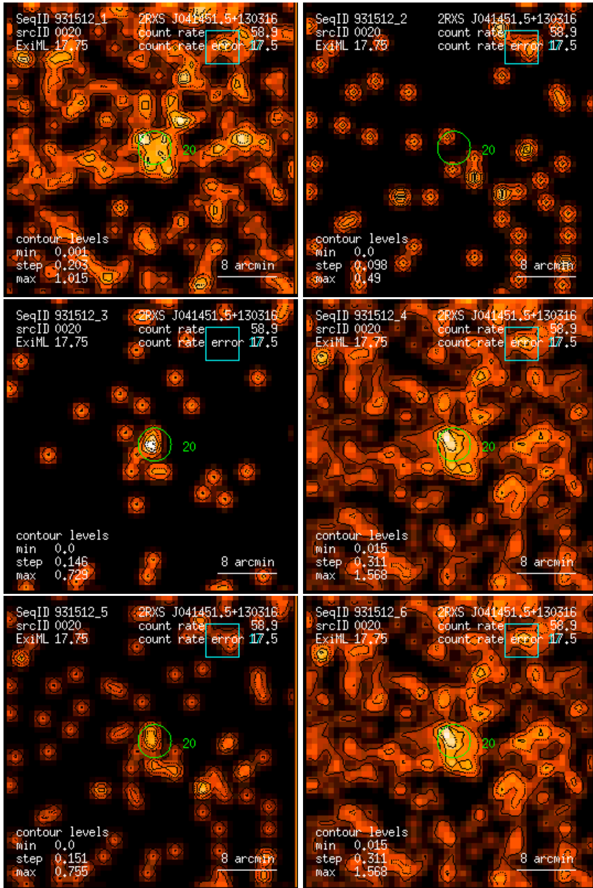
Figure 20: RASS 931512: detection 0020: band rate images, Gaussian filter: (1) PSPC channels 11 – 41, (2) 52 – 90, (3) 91 – 201, (4) 11 – 235, (5) 52 – 201, (6) 11 – 201. Broad band rates in counts/ks. Band rate contour levels in counts/ks/arcmin 2 .
