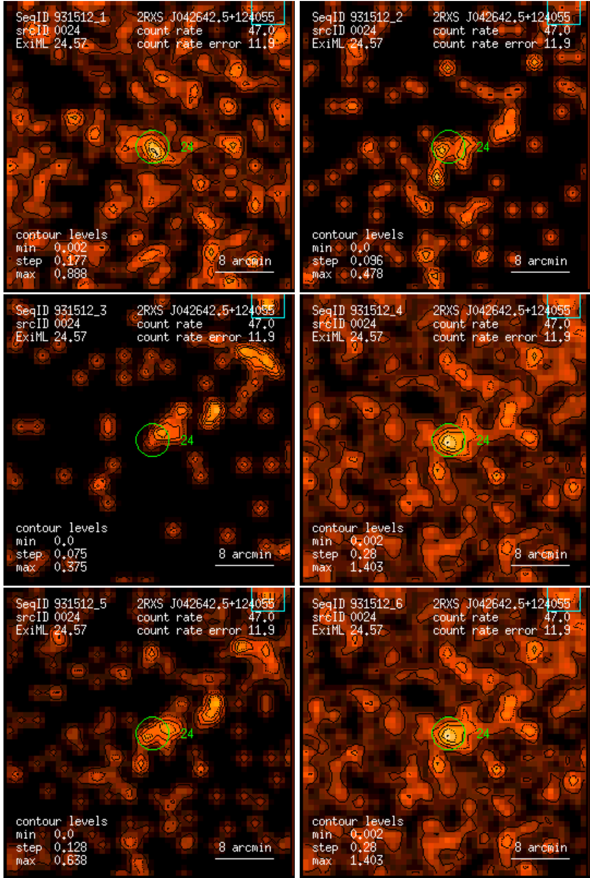
Figure 24: RASS 931512: detection 0024: band rate images, Gaussian filter: (1) PSPC channels 11 – 41, (2) 52 – 90, (3) 91 – 201, (4) 11 – 235, (5) 52 – 201, (6) 11 – 201. Broad band rates in counts/ks. Band rate contour levels in counts/ks/arcmin 2 .
