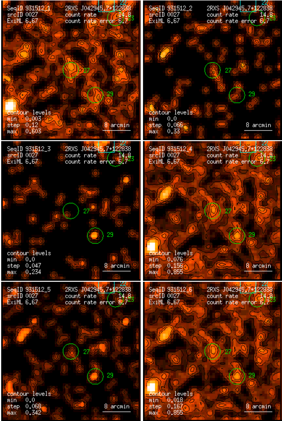
Figure 27: RASS 931512: detection 0027: band rate images, Gaussian filter: (1) PSPC channels 11 – 41, (2) 52 – 90, (3) 91 – 201, (4) 11 – 235, (5) 52 – 201, (6) 11 – 201. Broad band rates in counts/ks. Band rate contour levels in counts/ks/arcmin 2 .
