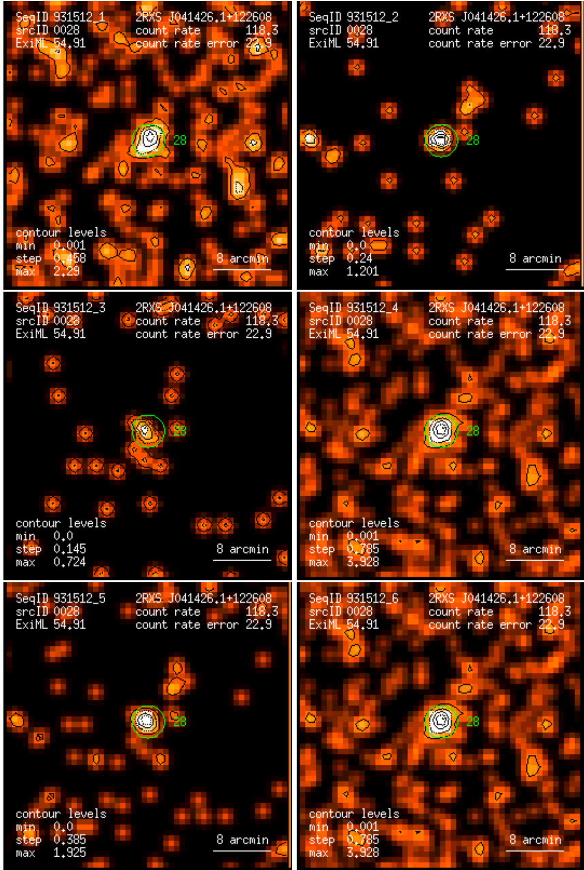
Figure 28: RASS 931512: detection 0028: band rate images, Gaussian filter: (1) PSPC channels 11 – 41, (2) 52 – 90, (3) 91 – 201, (4) 11 – 235, (5) 52 – 201, (6) 11 – 201. Broad band rates in counts/ks. Band rate contour levels in counts/ks/arcmin 2 .
