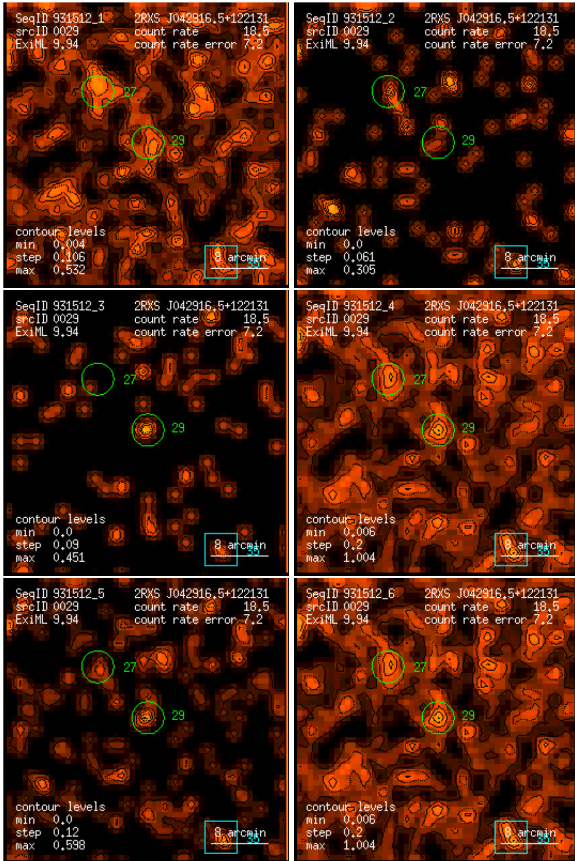
Figure 29: RASS 931512: detection 0029: band rate images, Gaussian filter: (1) PSPC channels 11 – 41, (2) 52 – 90, (3) 91 – 201, (4) 11 – 235, (5) 52 – 201, (6) 11 – 201. Broad band rates in counts/ks. Band rate contour levels in counts/ks/arcmin 2 .
