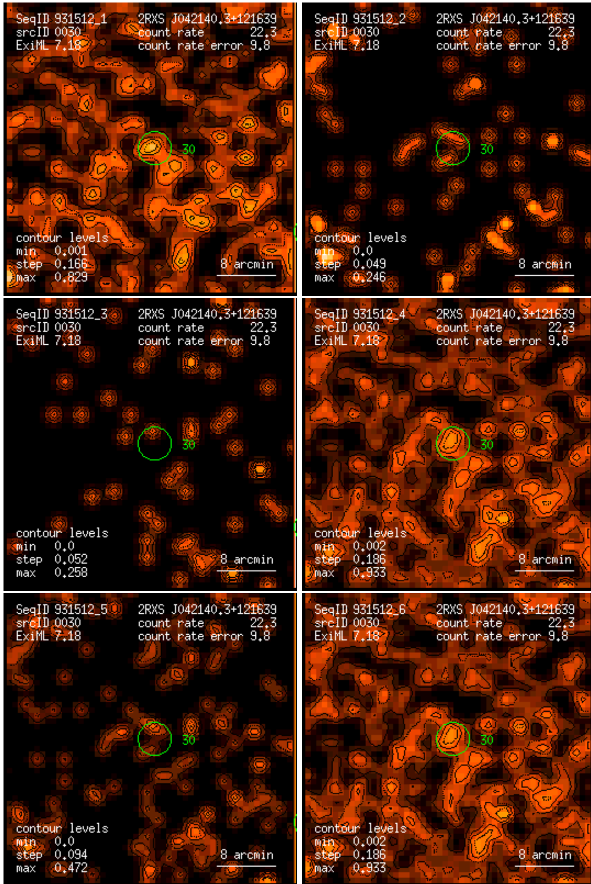
Figure 30: RASS 931512: detection 0030: band rate images, Gaussian filter: (1) PSPC channels 11 – 41, (2) 52 – 90, (3) 91 – 201, (4) 11 – 235, (5) 52 – 201, (6) 11 – 201. Broad band rates in counts/ks. Band rate contour levels in counts/ks/arcmin 2 .
