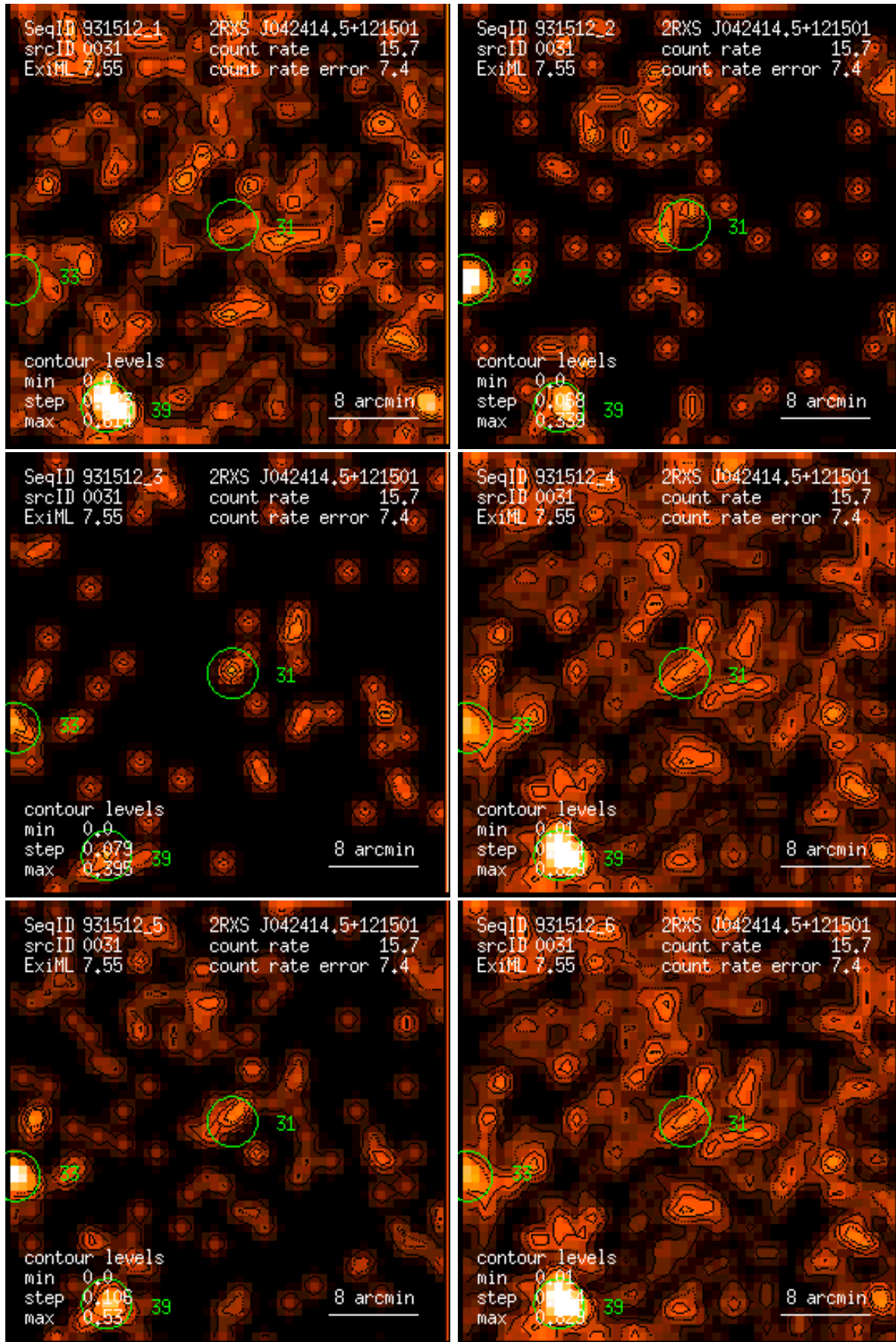
Figure 31: RASS 931512: detection 0031: band rate images, Gaussian filter: (1) PSPC channels 11 – 41, (2) 52 – 90, (3) 91 – 201, (4) 11 – 235, (5) 52 – 201, (6) 11 – 201. Broad band rates in counts/ks. Band rate contour levels in counts/ks/arcmin 2 .
