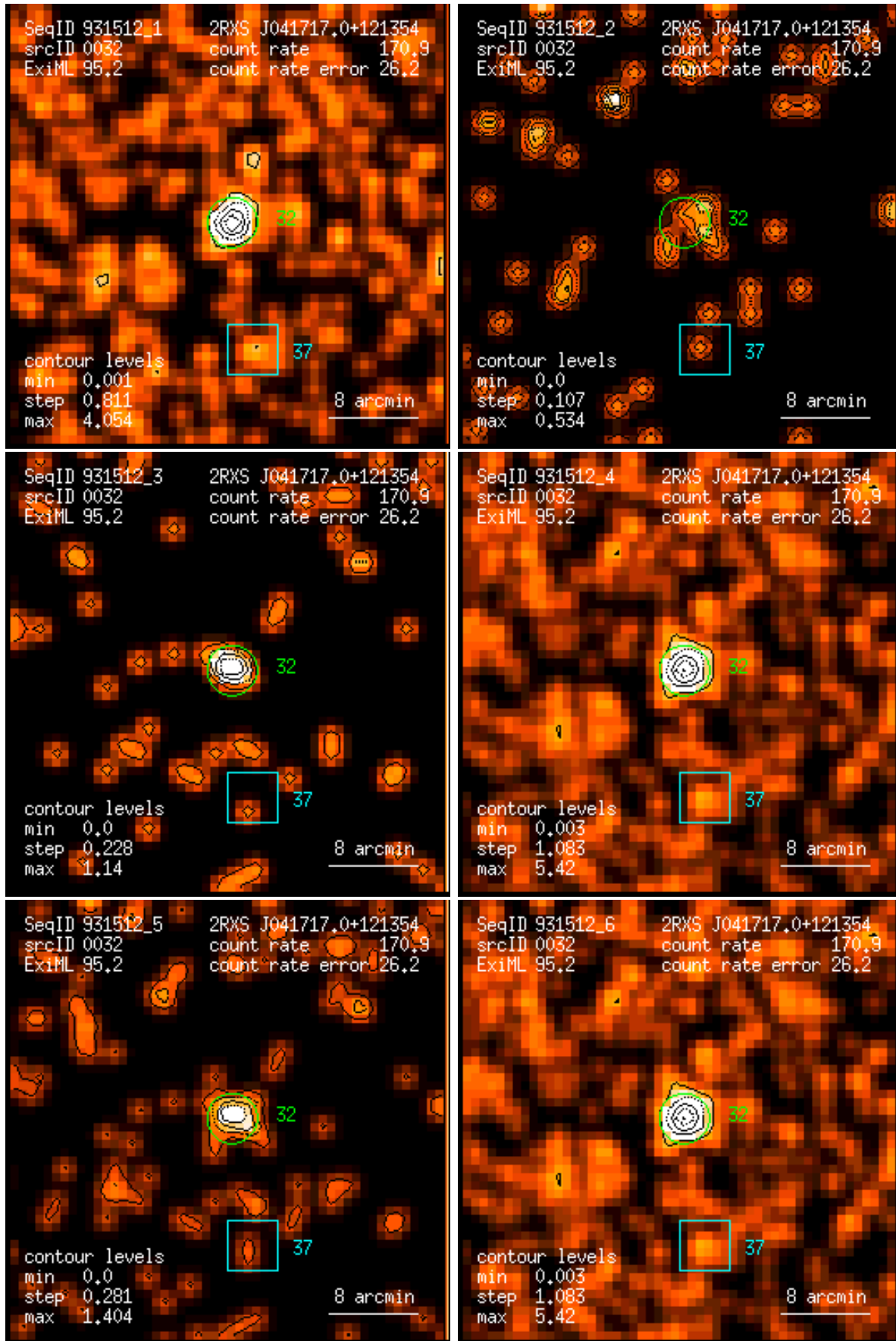
Figure 32: RASS 931512: detection 0032: band rate images, Gaussian filter: (1) PSPC channels 11 – 41, (2) 52 – 90, (3) 91 – 201, (4) 11 – 235, (5) 52 – 201, (6) 11 – 201. Broad band rates in counts/ks. Band rate contour levels in counts/ks/arcmin 2 .
