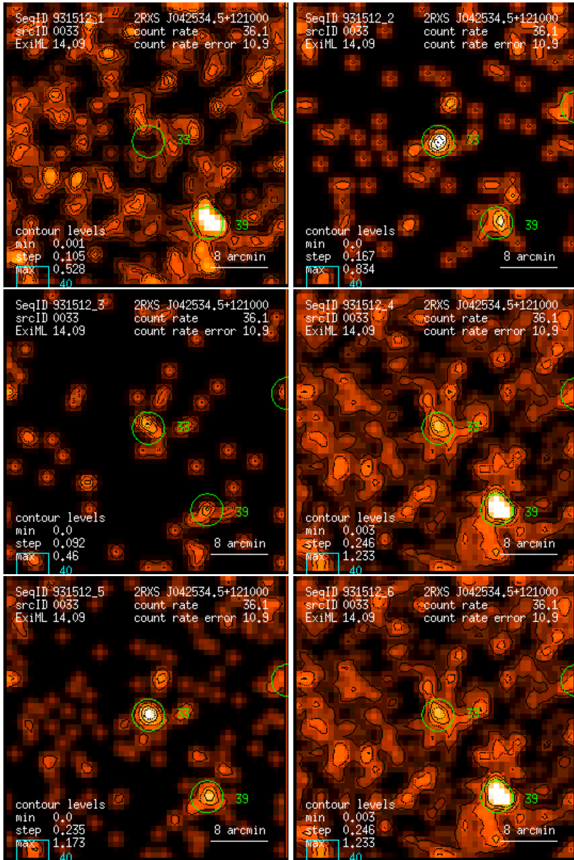
Figure 33: RASS 931512: detection 0033: band rate images, Gaussian filter: (1) PSPC channels 11 – 41, (2) 52 – 90, (3) 91 – 201, (4) 11 – 235, (5) 52 – 201, (6) 11 – 201. Broad band rates in counts/ks. Band rate contour levels in counts/ks/arcmin 2 .
