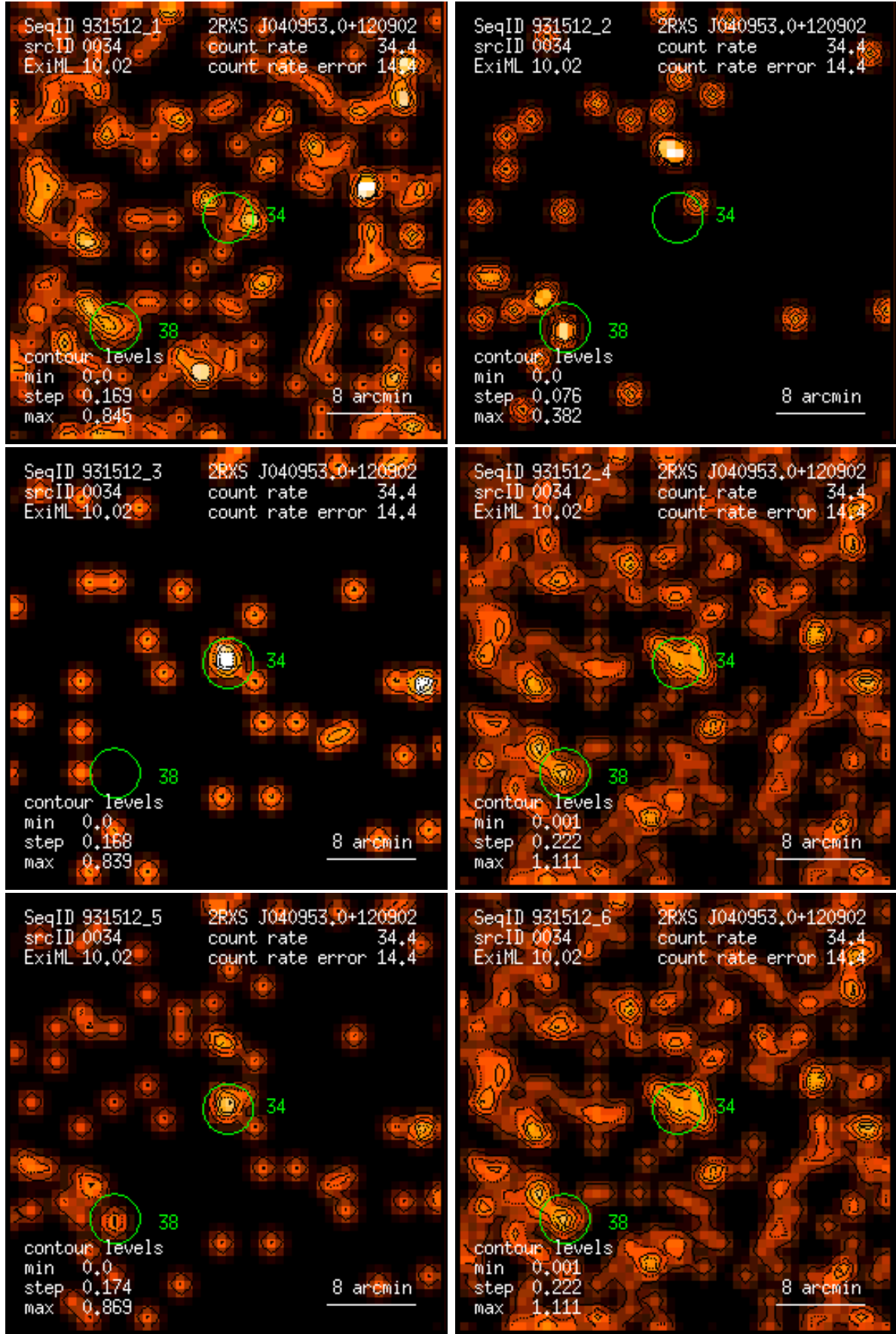
Figure 34: RASS 931512: detection 0034: band rate images, Gaussian filter: (1) PSPC channels 11 – 41, (2) 52 – 90, (3) 91 – 201, (4) 11 – 235, (5) 52 – 201, (6) 11 – 201. Broad band rates in counts/ks. Band rate contour levels in counts/ks/arcmin 2 .
