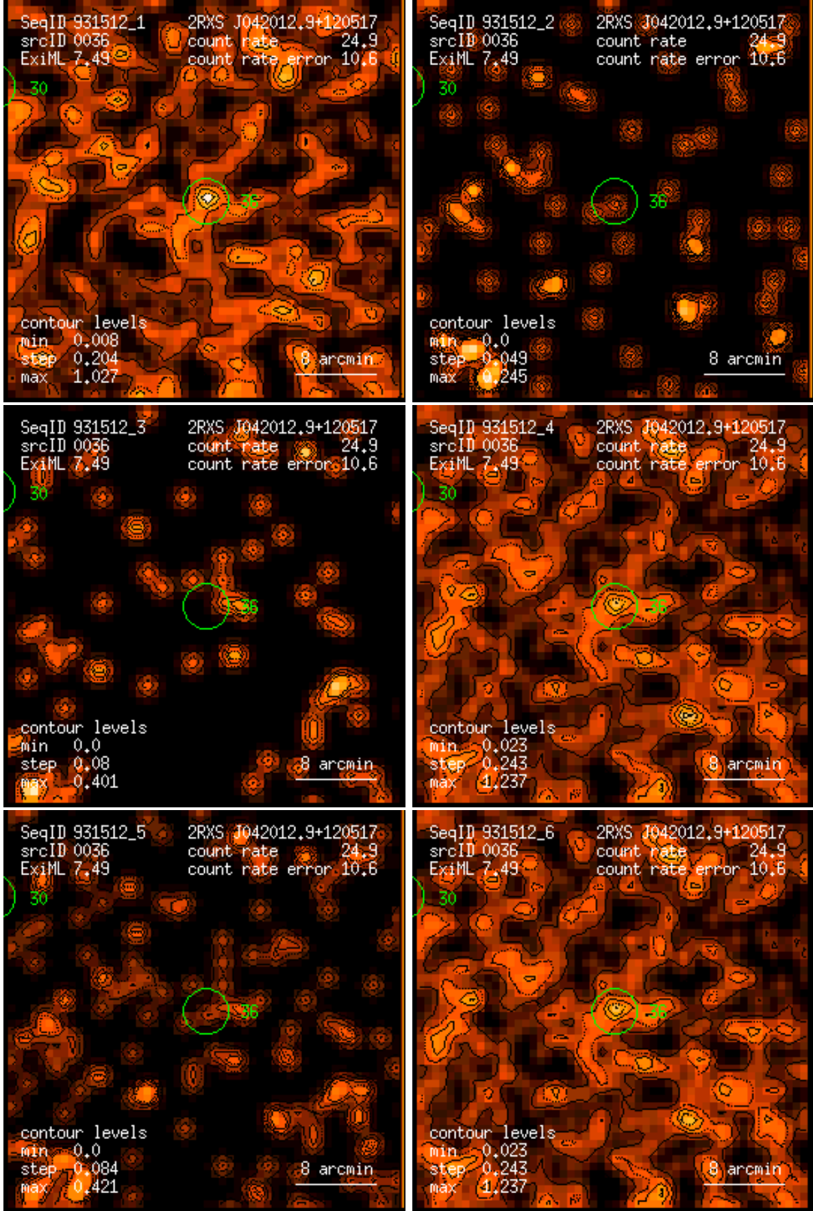
Figure 36: RASS 931512: detection 0036: band rate images, Gaussian filter: (1) PSPC channels 11 – 41, (2) 52 – 90, (3) 91 – 201, (4) 11 – 235, (5) 52 – 201, (6) 11 – 201. Broad band rates in counts/ks. Band rate contour levels in counts/ks/arcmin 2 .
