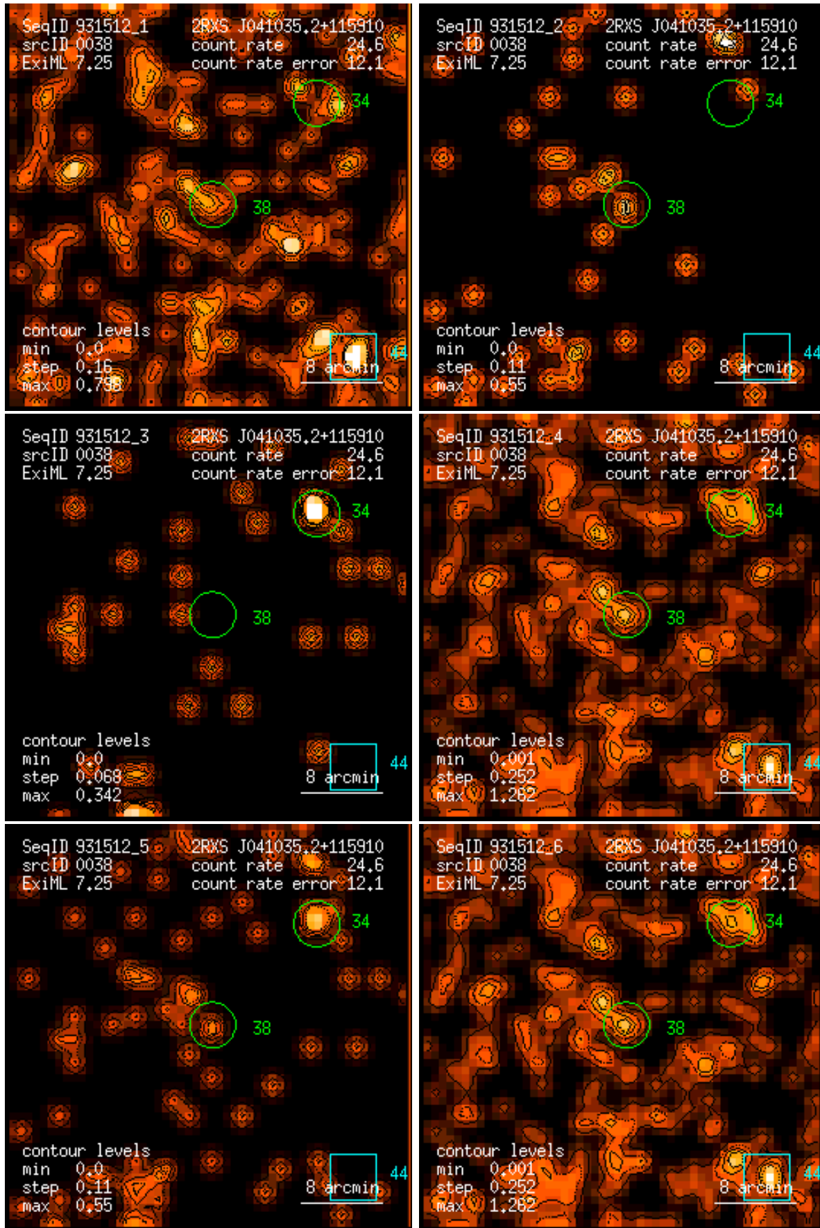
Figure 38: RASS 931512: detection 0038: band rate images, Gaussian filter: (1) PSPC channels 11 – 41, (2) 52 – 90, (3) 91 – 201, (4) 11 – 235, (5) 52 – 201, (6) 11 – 201. Broad band rates in counts/ks. Band rate contour levels in counts/ks/arcmin 2 .
