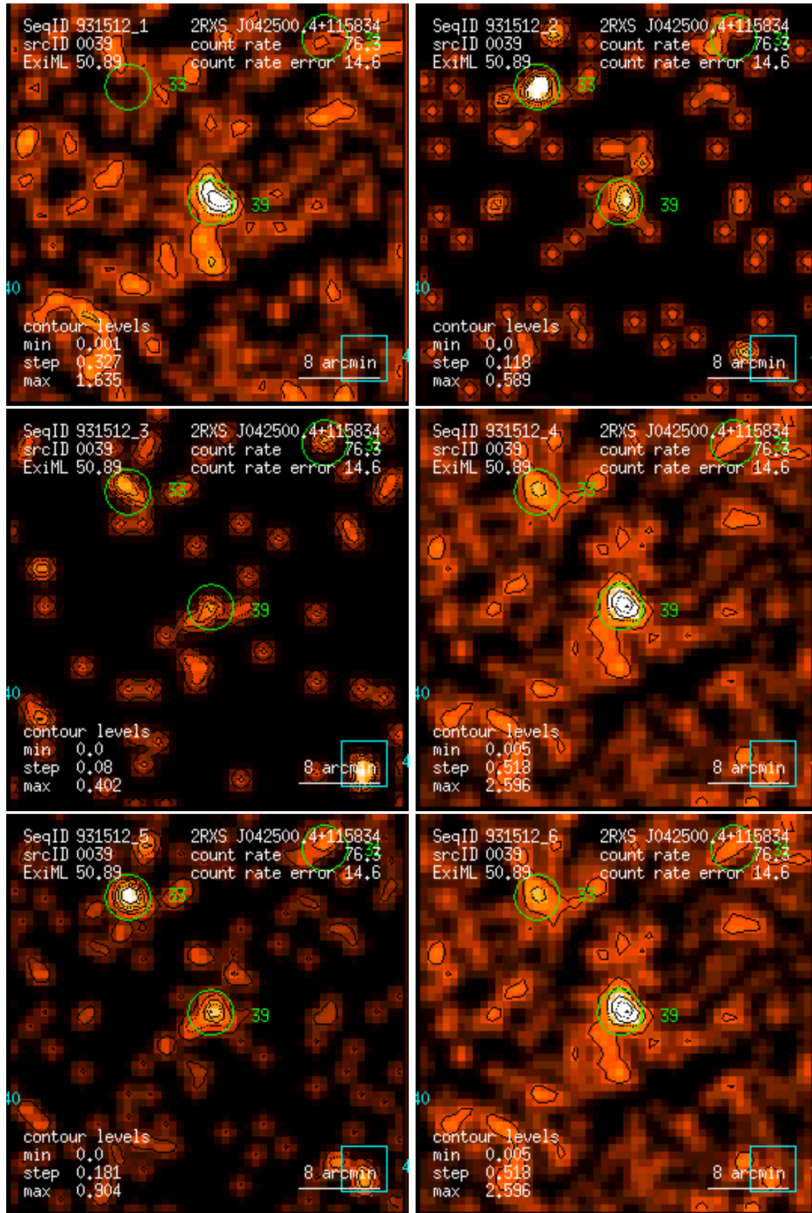
Figure 39: RASS 931512: detection 0039: band rate images, Gaussian filter: (1) PSPC channels 11 – 41, (2) 52 – 90, (3) 91 – 201, (4) 11 – 235, (5) 52 – 201, (6) 11 – 201. Broad band rates in counts/ks. Band rate contour levels in counts/ks/arcmin 2 .
