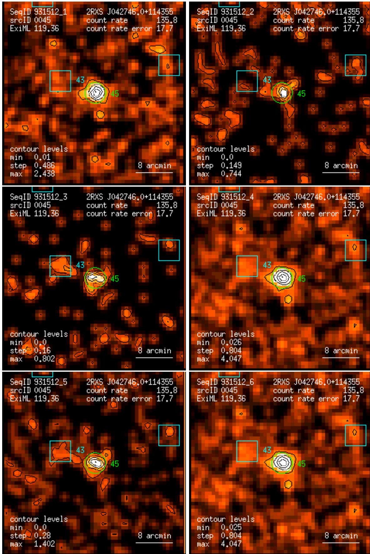
Figure 45: RASS 931512: detection 0045: band rate images, Gaussian filter: (1) PSPC channels 11 – 41, (2) 52 – 90, (3) 91 – 201, (4) 11 – 235, (5) 52 – 201, (6) 11 – 201. Broad band rates in counts/ks. Band rate contour levels in counts/ks/arcmin 2 .
