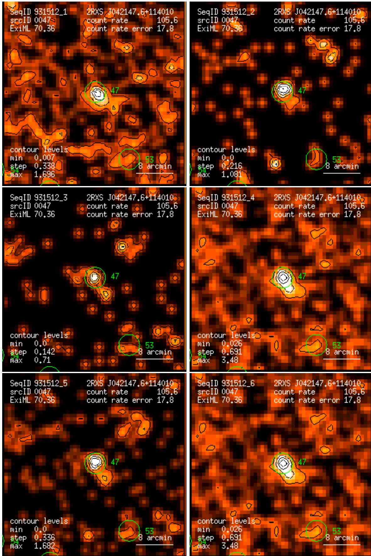
Figure 47: RASS 931512: detection 0047: band rate images, Gaussian filter: (1) PSPC channels 11 – 41, (2) 52 – 90, (3) 91 – 201, (4) 11 – 235, (5) 52 – 201, (6) 11 – 201. Broad band rates in counts/ks. Band rate contour levels in counts/ks/arcmin 2 .
