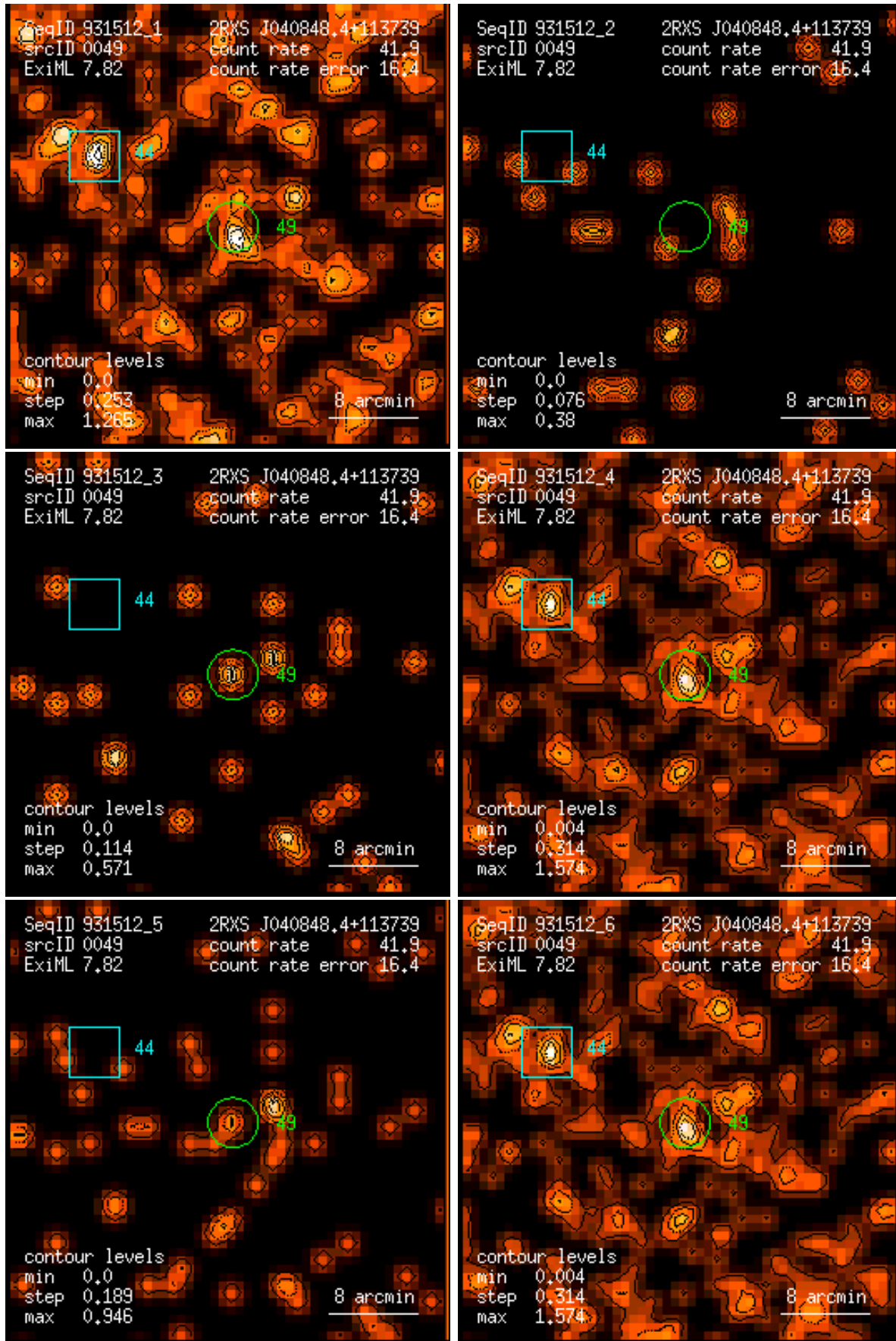
Figure 49: RASS 931512: detection 0049: band rate images, Gaussian filter: (1) PSPC channels 11 – 41, (2) 52 – 90, (3) 91 – 201, (4) 11 – 235, (5) 52 – 201, (6) 11 – 201. Broad band rates in counts/ks. Band rate contour levels in counts/ks/arcmin 2 .
