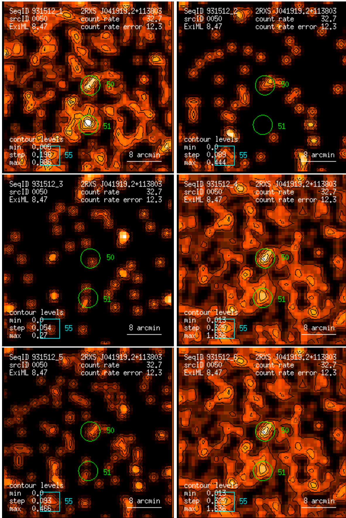
Figure 50: RASS 931512: detection 0050: band rate images, Gaussian filter: (1) PSPC channels 11 – 41, (2) 52 – 90, (3) 91 – 201, (4) 11 – 235, (5) 52 – 201, (6) 11 – 201. Broad band rates in counts/ks. Band rate contour levels in counts/ks/arcmin 2 .
