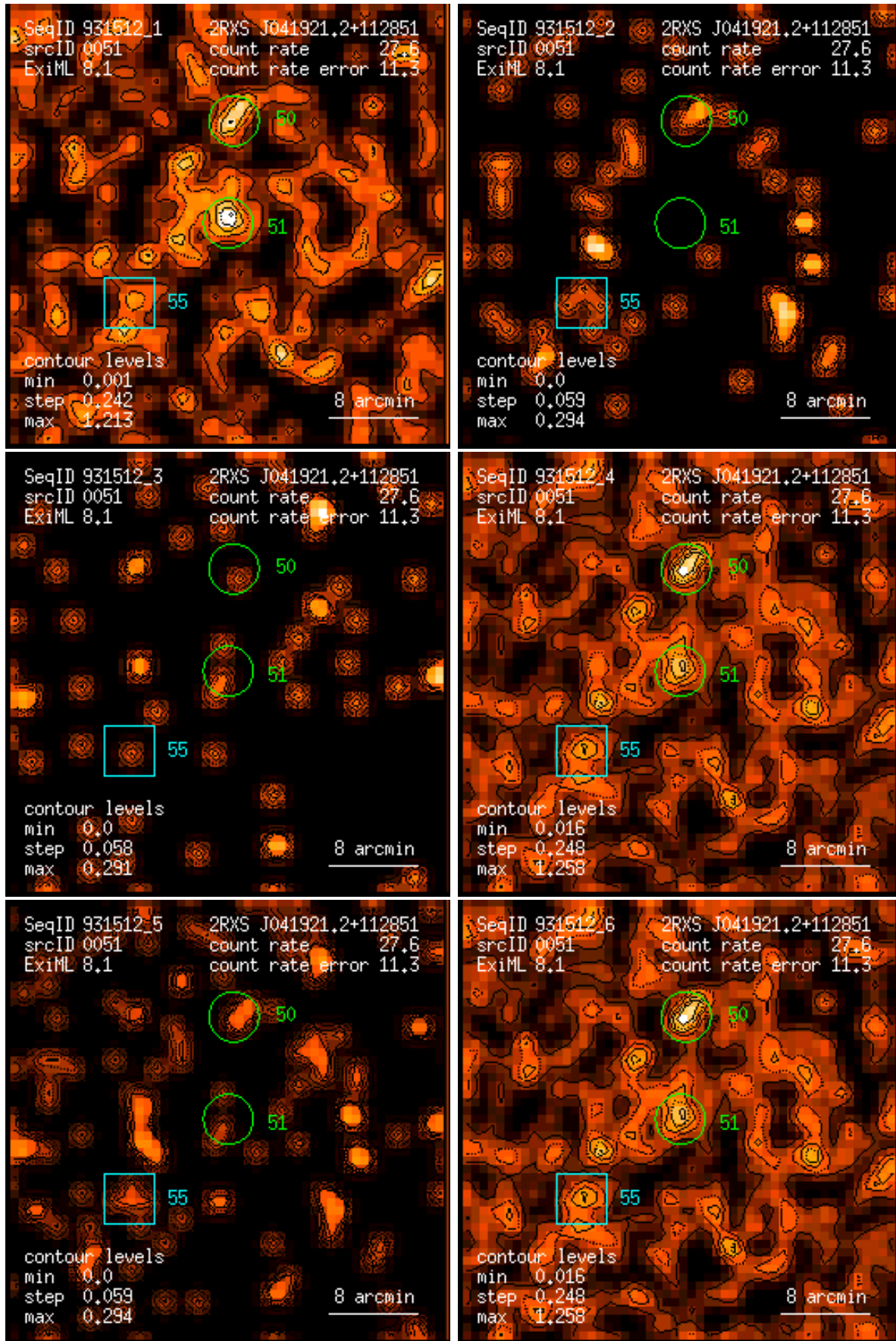
Figure 51: RASS 931512: detection 0051: band rate images, Gaussian filter: (1) PSPC channels 11 – 41, (2) 52 – 90, (3) 91 – 201, (4) 11 – 235, (5) 52 – 201, (6) 11 – 201. Broad band rates in counts/ks. Band rate contour levels in counts/ks/arcmin 2 .
