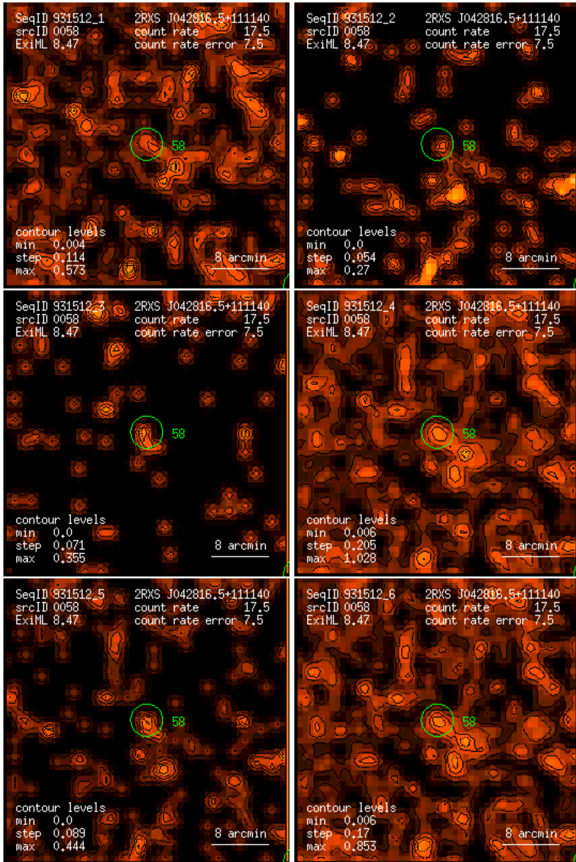
Figure 58: RASS 931512: detection 0058: band rate images, Gaussian filter: (1) PSPC channels 11 – 41, (2) 52 – 90, (3) 91 – 201, (4) 11 – 235, (5) 52 – 201, (6) 11 – 201. Broad band rates in counts/ks. Band rate contour levels in counts/ks/arcmin 2 .
