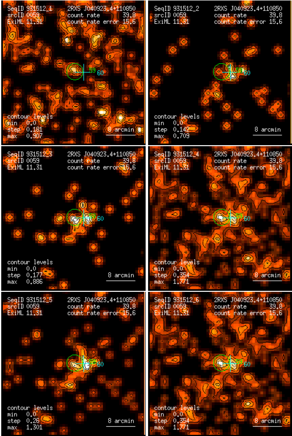
Figure 59: RASS 931512: detection 0059: band rate images, Gaussian filter: (1) PSPC channels 11 – 41, (2) 52 – 90, (3) 91 – 201, (4) 11 – 235, (5) 52 – 201, (6) 11 – 201. Broad band rates in counts/ks. Band rate contour levels in counts/ks/arcmin 2 .
