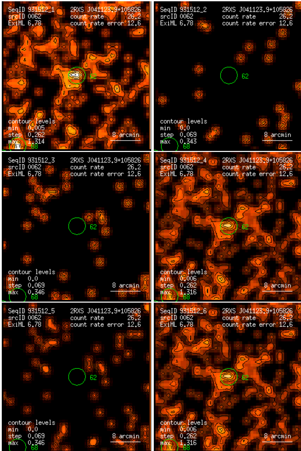
Figure 62: RASS 931512: detection 0062: band rate images, Gaussian filter: (1) PSPC channels 11 – 41, (2) 52 – 90, (3) 91 – 201, (4) 11 – 235, (5) 52 – 201, (6) 11 – 201. Broad band rates in counts/ks. Band rate contour levels in counts/ks/arcmin 2 .
