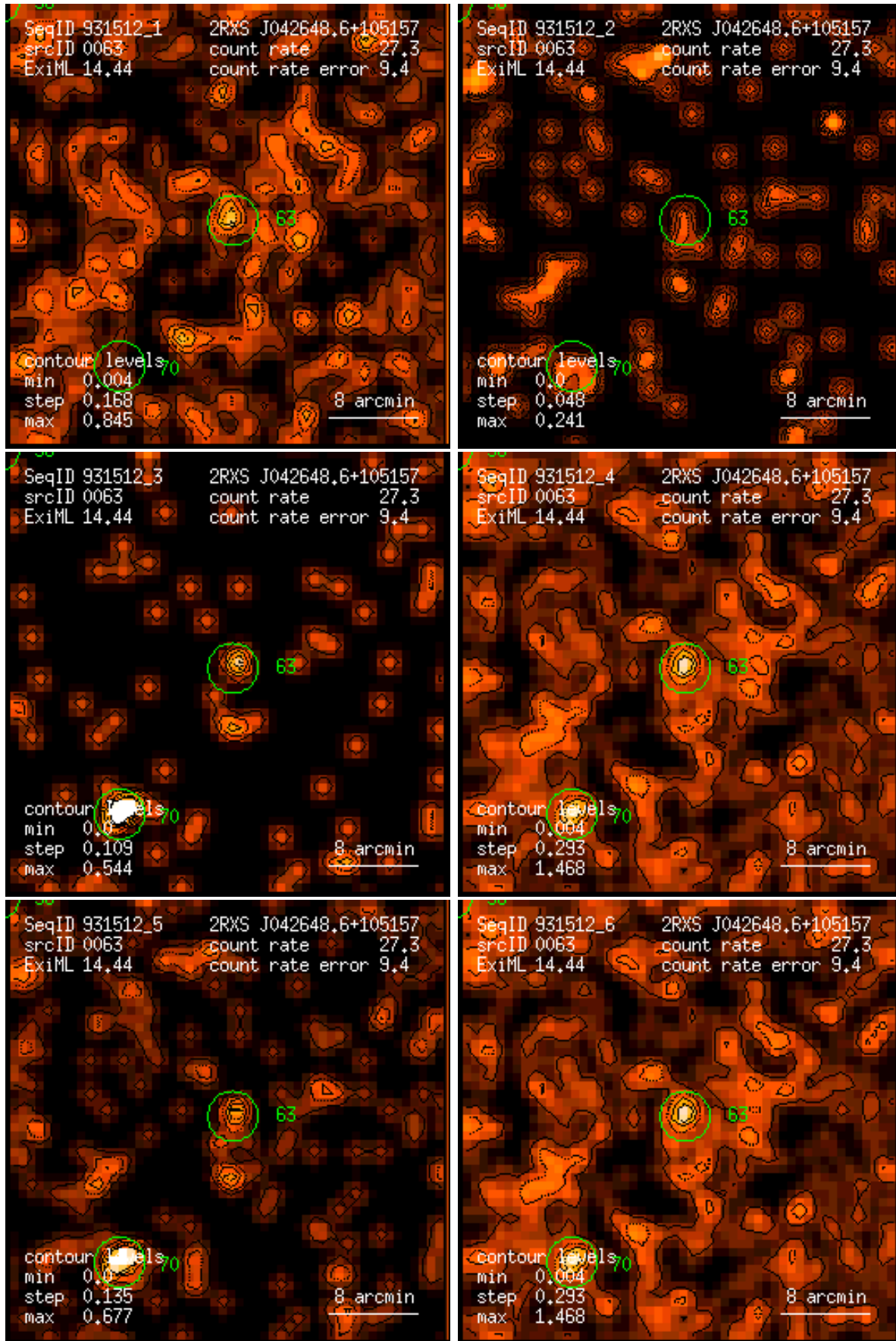
Figure 63: RASS 931512: detection 0063: band rate images, Gaussian filter: (1) PSPC channels 11 – 41, (2) 52 – 90, (3) 91 – 201, (4) 11 – 235, (5) 52 – 201, (6) 11 – 201. Broad band rates in counts/ks. Band rate contour levels in counts/ks/arcmin 2 .
